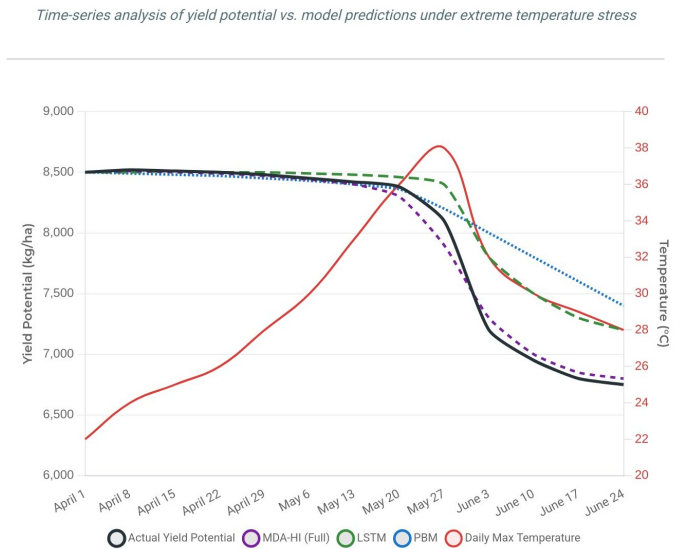
Figure 6. Model Performance During the 2025 Hebei Heatwave.
