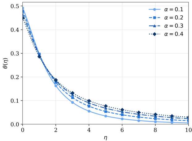
Figure 8. Temperature profile \theta(\eta) for different values of the curvature parameter \alpha ( \beta = 0.1 , M = 0.2 , Po = 0.2 , Pr = 1 , Ec = 0.2 , \gamma = 0.1 ).
