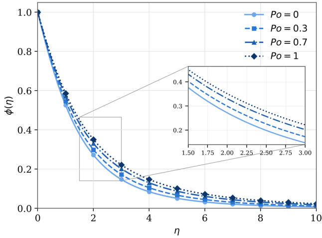
Figure 5. Concentration profile \phi(\eta) for different values of the porous-medium parameter Po ( \beta = 0.1 , M = 0.2 , \alpha = 0.1 , Sc = 1 ); the inset enlarges 1.5 \leq \eta \leq 3 .
