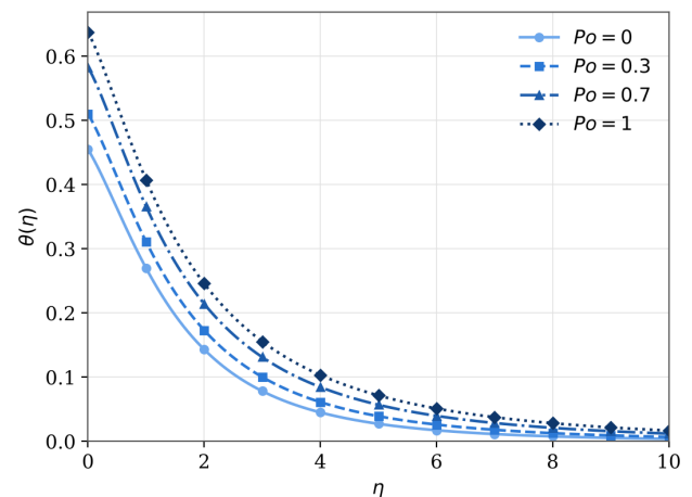
Figure 4. Temperature profile \theta(\eta) for different values of the porous-medium parameter Po ( \beta = 0.1 , M = 0.2 , \alpha = 0.1 , Pr = 1 , Ec = 0.2 , \gamma = 0.1 ).
