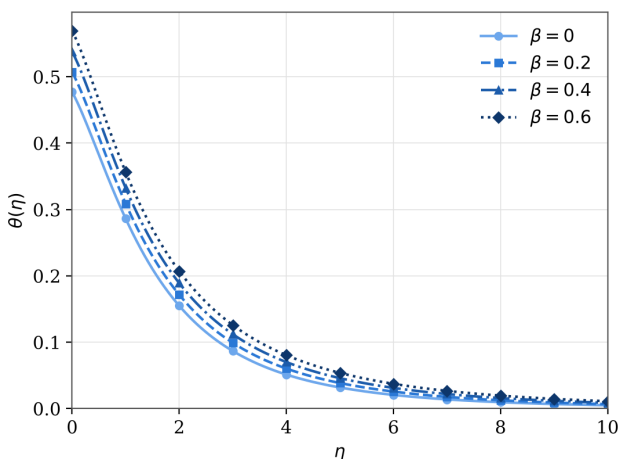
Figure 6. Temperature profile \theta(\eta) for different values of the Maxwell parameter \beta ( M = 0.2 , \alpha = 0.1 , Po = 0.2 , Pr = 1 , Ec = 0.2 , \gamma = 0.1 ).
