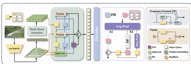
Figure 4. UAV-DETR: a transformer-based object-detection model for UAV aerial images. Reproduced from Ref. [41]. The framework incorporates a multi-scale feature-fusion module with frequency enhancement, a frequency-focused downsampling module, and a semantic-alignment and calibration module to balance spatial and frequency information at different scales.
