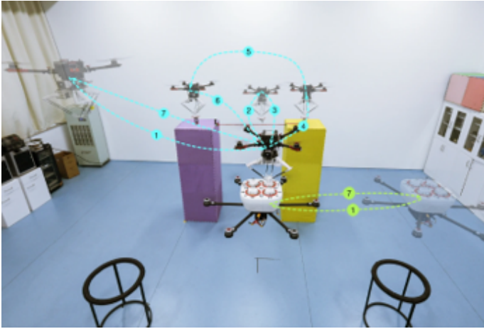
Figure 6. FlyingToolbox, a cooperative aerial manipulation system with sub-centimetre-level docking accuracy under vertical-stack flight conditions, suggesting a new model for heterogeneous and interactive flying robot cooperation in diverse applications. Reproduced from Ref. [84].
