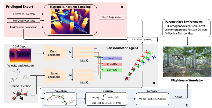
Figure 5. An end-to-end approach for high-speed autonomous quadrotor flight with onboard sensing and computation. Reproduced from Ref. [52]. The method learns a sensorimotor mapping with a convolutional network trained in simulation through privileged learning.
