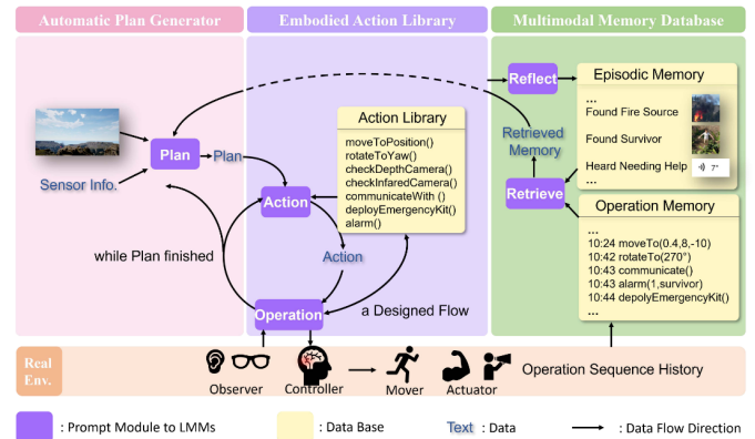
Figure 9. AeroAgent, an agent framework tailored for industrial drone technology that harnesses the power of Large Multimodal Models (LMMs), outperforms existing Deep Reinforcement Learning (DRL)-based agents in experimental evaluations, which highlights the advantages of embodied LMMs in complex real-world scenarios. Reproduced from Ref. [58].
