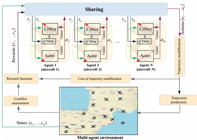
Figure 8. A cooperative decision-making framework using multi-agent deep reinforcement learning for operationally feasible climate-friendly trajectory planning. Reproduced from Ref. [57] under the CC BY-NC-ND 4.0 license. The framework uses twin delayed deep deterministic policy gradient (TD3) to adjust trajectories and resolve potential conflicts associated with climate-optimal routes.
