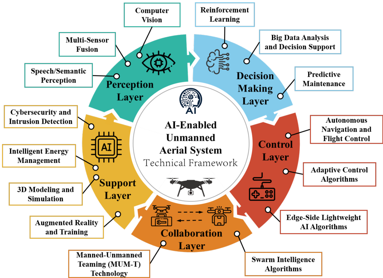
Figure 3. The core technical framework of AI-enabled aerial unmanned systems. Source: created by the authors.
