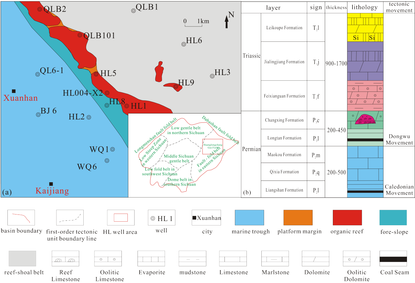
Figure 1. (a) Tectonic location, well distribution and sedimentary facies of the study area; (b) Stratigraphic column from Liangshan Formation to Leikoupo Formation.
