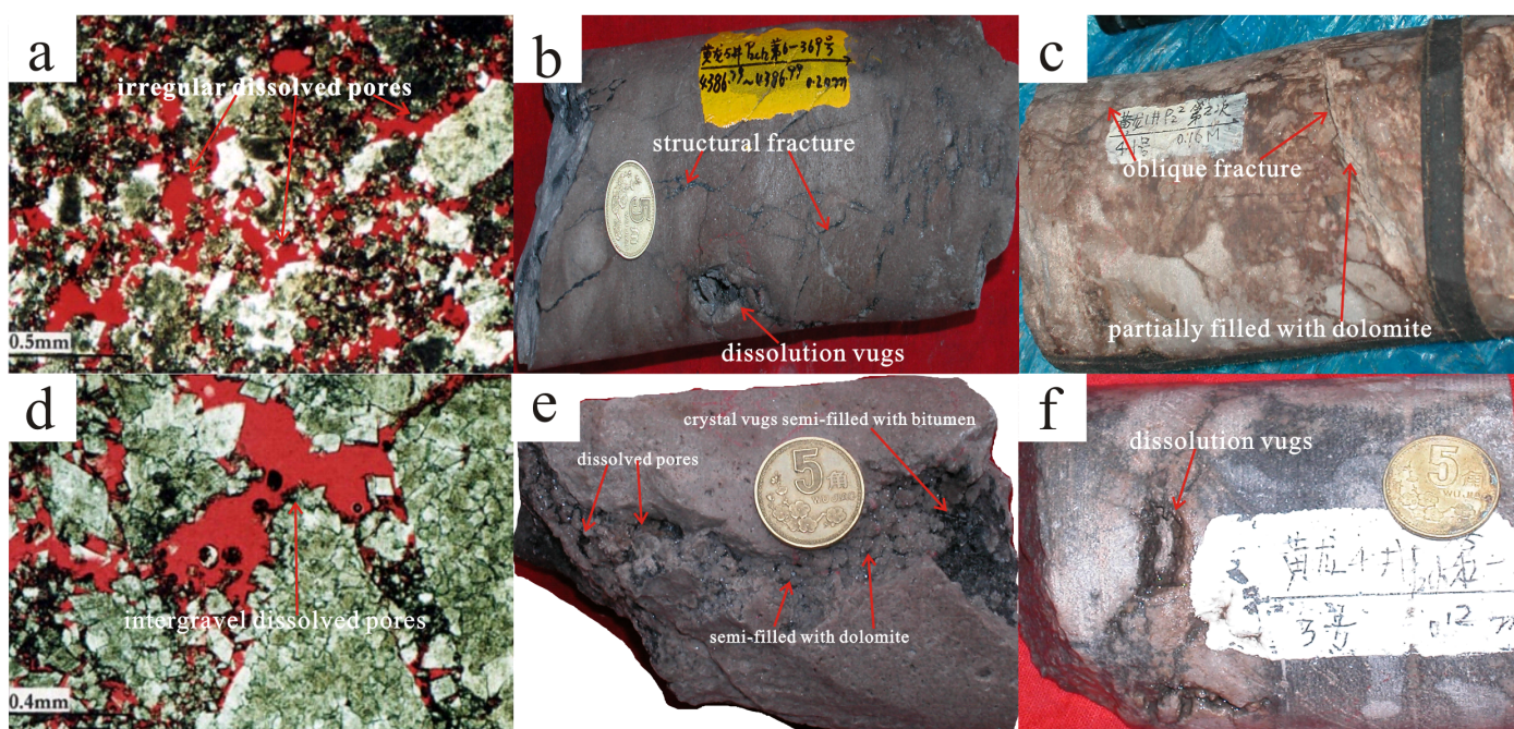
Figure 2. Core photographs and polarized-light photomicrographs of the Changxing Formation in HL wellfield. (a) A red cast thin-section photomicrograph shows well-developed irregular dissolved pores in dolomite, sample depth 4361.35 m. (b) Peloidal dolomite core developed with abundant fractures and dissolution vugs, sample depth 4386.29–4386.99 m. (c) Reef breccia dolomite develops oblique fractures partially filled with dolomite, sample depth 4241.12–4241.28 m. (d) A red cast thin section presents intense dissolution and developed intergranular/interclast dissolution pores in rudstone dolomite, sample depth 4232.21 m. (e) Dolomite core develops dissolved pores and crystal vugs semi-filled with dolomite and bitumen, sample depth 4376.31–4376.45 m. (f) Rudstone dolomite core characterized by widely developed dissolution vugs inside rocks, sample depth 4366.11–4366.23 m.
