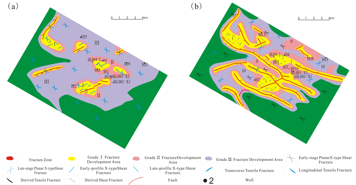
Figure 6. Rock failure degree zonation map of the Changxing Formation in Huanglong field for different stages. (a) Stage I; (b) Stage II.
