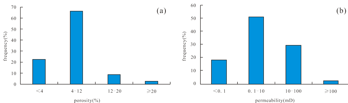
Figure 3. Histogram illustrating the statistical analysis of physical properties for core samples from the Changxing Formation in the Huanglongchang area. Panel (a) displays the distribution of the measured porosity values, while panel (b) shows the distribution of permeability values.
