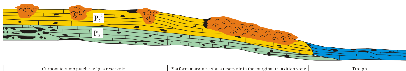
Figure 4. Sedimentary model of the Changxing Formation, Huanglongchang Block.
