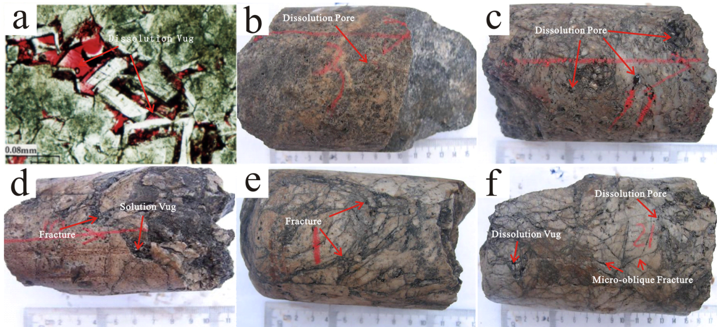
Figure 7. Microscopic photographs and hand specimen & core characteristics of syndepositional-supergene karst in the Changxing Formation, Huanglongchang area. (a) Microphotograph of rudstone dolomite with moldic pores; Well HL1, sampling depth 3957.6 m. (b) Dark gray finely crystalline vuggy dolomite with abundant dissolution pores and vugs; Well HL004-2, sampling depth 3490.05–3490.13 m. (c) Gray finely crystalline vuggy dolomite with well-developed but unevenly distributed dissolution pores and vugs; the plane porosity generally ranges from 1% to 3%, locally up to 3%–5%. A total of 262 small vugs, 92 medium vugs and 12 large vugs are identified, with euhedral calcite crystals observed on the wall of individual vugs; Well HL004-2, sampling depth 3490.93–3491.03 m. (d) Micritic dolomite with well-developed vugs and dissolution pores, as well as effective fractures and microfractures that mutually intersect; Well HL4, sampling depth 3509.89–3509.99 m. (e) Dark gray finely crystalline vuggy dolomite developed with horizontal and oblique microfractures; these fractures intersect to form a reticular network, and most pores, fractures and vugs are interconnected; Well HL5, sampling depth 4332.8–4332.93 m. (f) Light brownish-gray finely crystalline vuggy dolomite with abundant oblique microfractures intersecting small effective oblique and vertical fractures to form a reticular network; most pores, fractures and vugs are interconnected, and gas bleeding is detected at 42 pore-fracture points; Well HL8, sampling depth 3551.23–3551.33 m.
