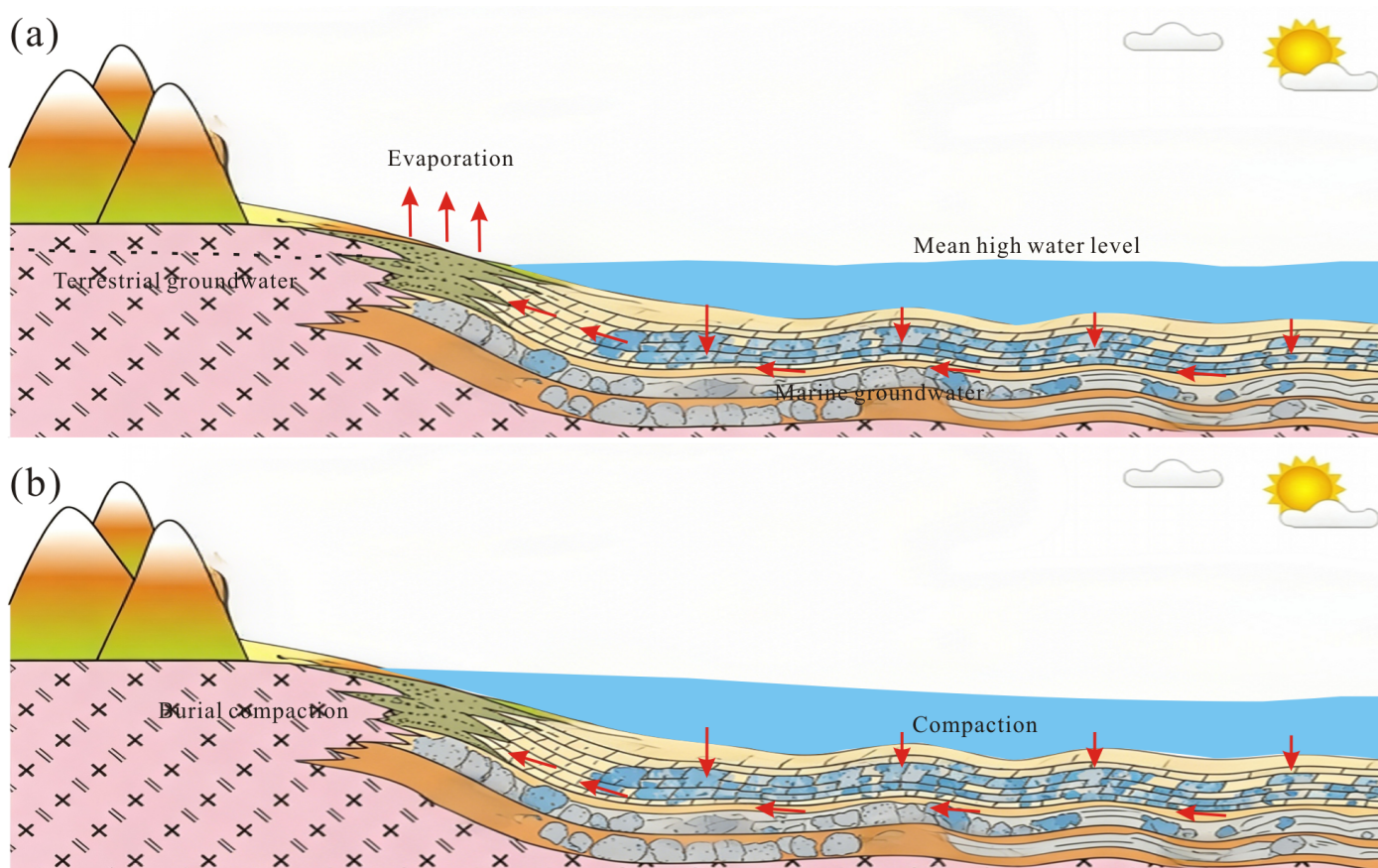
Figure 5. Genetic model of dolomitization for the Changxing Formation in the Huanglongchang area. (a) Evaporative pumping dolomitization model; (b) Burial dolomitization model.
