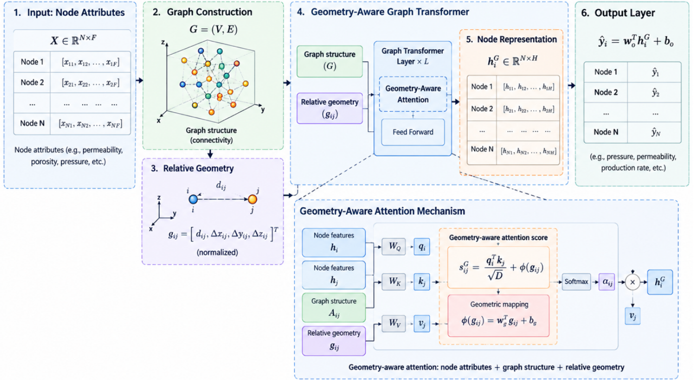
Figure 2. Architecture of the Geometry-Aware Graph Transformer (GAGT). Node attributes, graph structure, and relative geometric information are combined through a learnable geometric bias in the attention mechanism to produce geometry-aware node representations.
