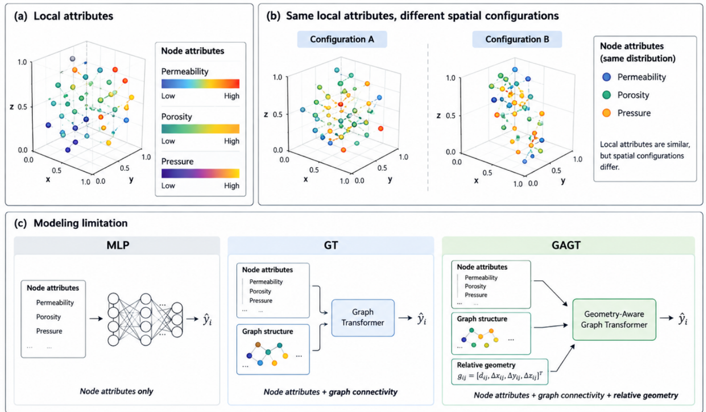
Figure 1. Problem definition and motivation for geometry-aware learning. (a) Local node attributes in an irregular three-dimensional subsurface setting. (b) Spatial configurations with similar local attributes but different relative spatial relationships. (c) Information inputs used by the MLP, Graph Transformer (GT), and Geometry-Aware Graph Transformer (GAGT).
