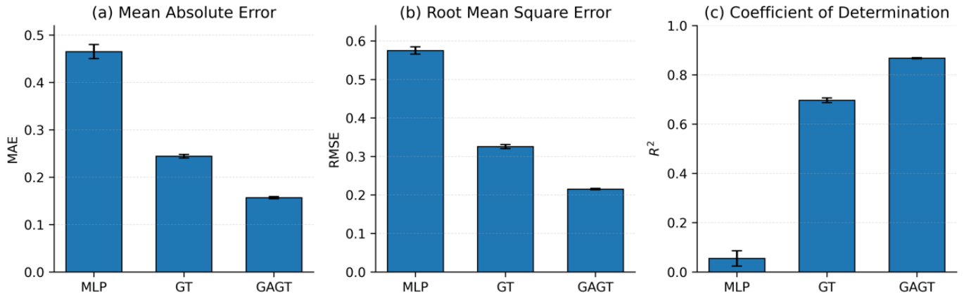
Figure 3. Test-set (a) MAE, (b) RMSE, and (c) R^2 of MLP, Graph Transformer (GT), and Geometry-Aware Graph Transformer (GAGT) over 10 random seeds. Error bars indicate the standard deviation across seeds.
