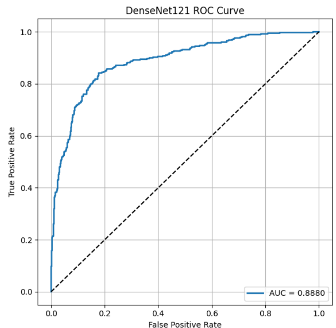
Figure 4. ROC curve for the DenseNet121 model.
