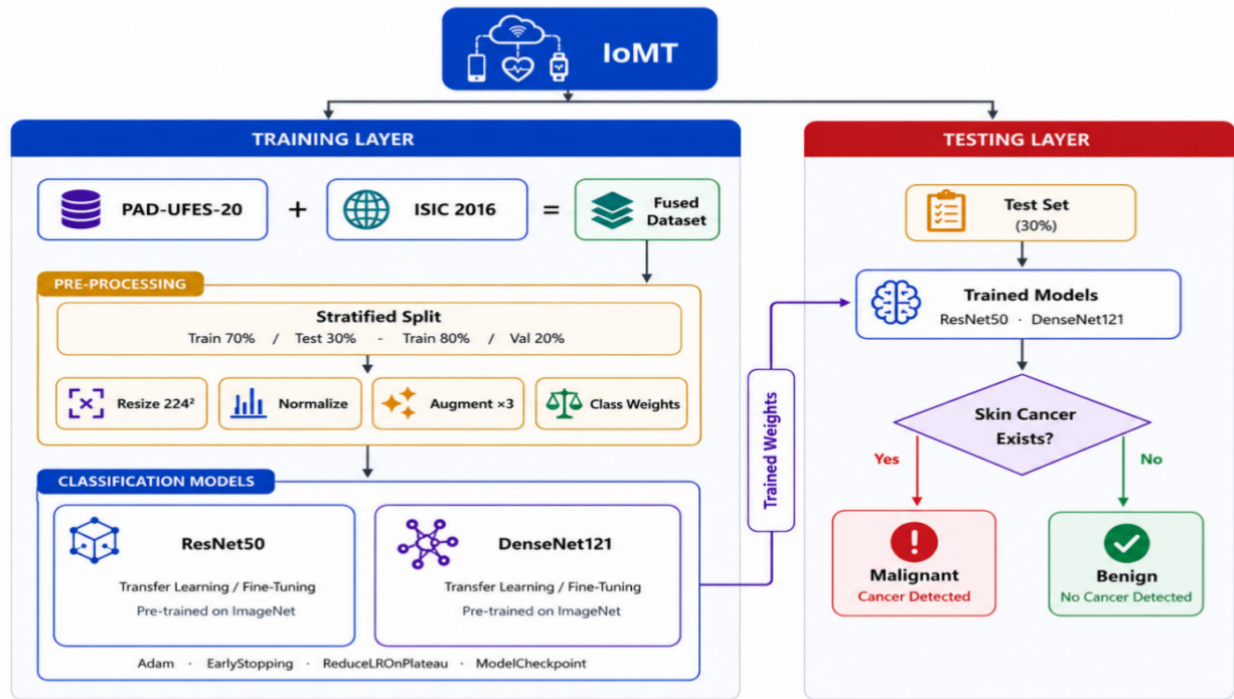
Figure 2. Proposed framework for binary skin cancer classification.
