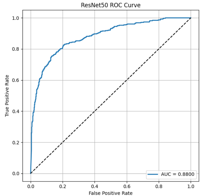
Figure 3. ROC curve for the ResNet50 model.
