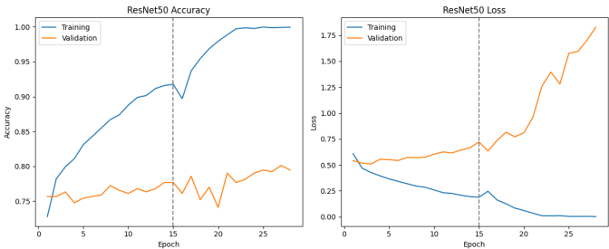
Figure 5. Training and validation accuracy and loss curves for ResNet50.
