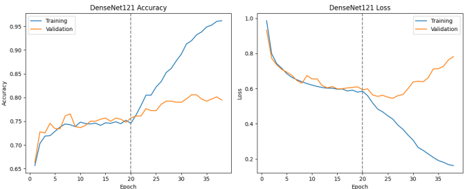
Figure 6. Training and validation accuracy and loss curves for DenseNet121.
