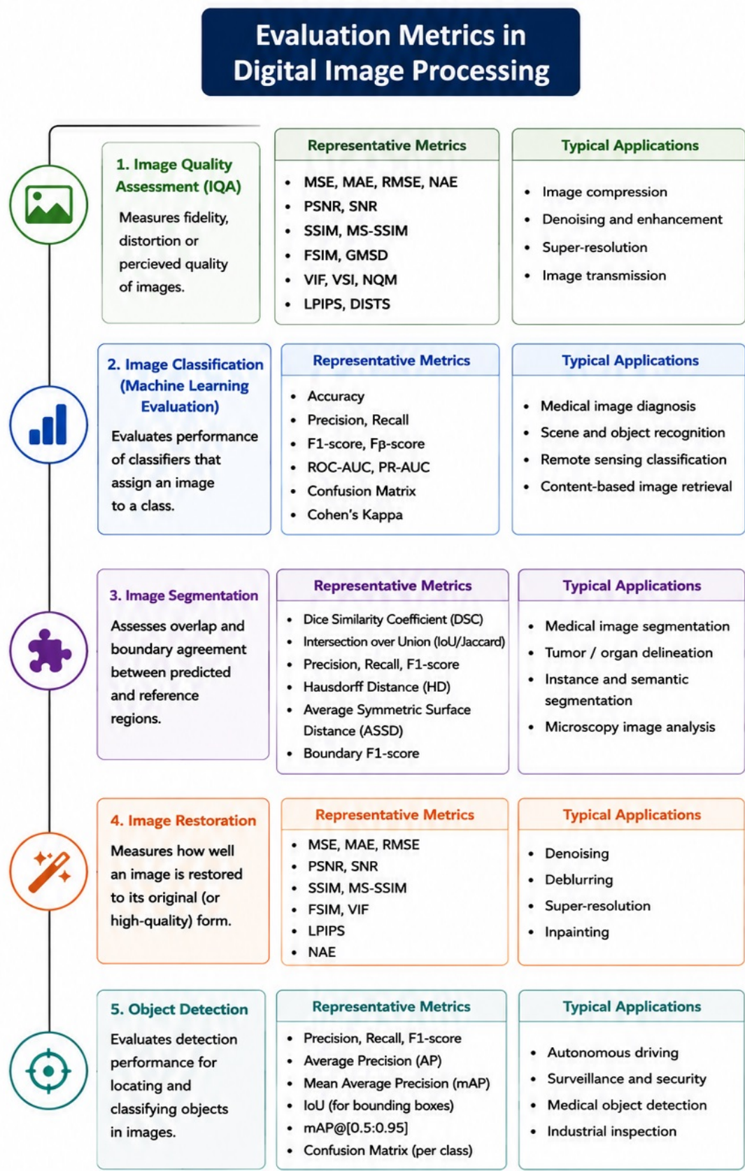
Figure 1. Taxonomy of evaluation metrics for digital image processing.
