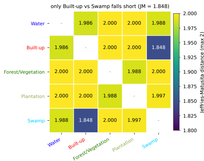
Figure 13. Pairwise class separability (JM distance) plotted against the conventional threshold of 1.9. Only built-up against swamp falls short, at 1.848.
