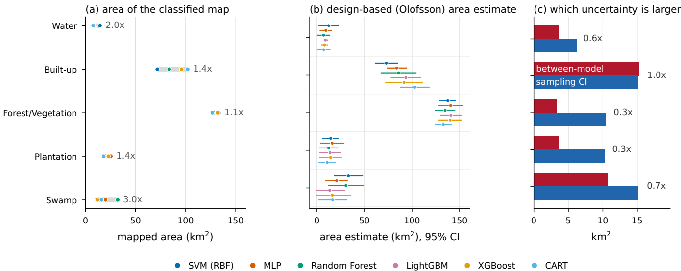
Figure 11. Between-model area uncertainty. (a) Mapped area of each class in each of the six maps, annotated with the ratio of largest to smallest. (b) Design-based area estimates with 95% intervals, computed per model after Olofsson et al. [35]. (c) For each class, half the between-model range (red) against the median single-model 95% half-width (blue); the annotated ratio is red divided by blue.
