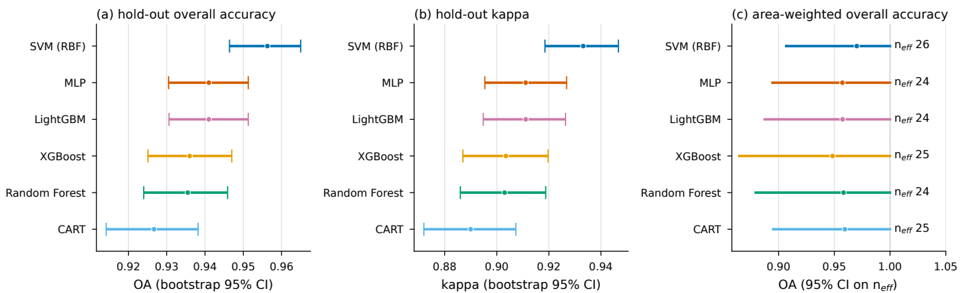
Figure 8. Model accuracy with uncertainty. (a) Hold-out overall accuracy and (b) hold-out \kappa , with 2,000-replicate bootstrap 95% intervals over the 1,829 validation pixels. (c) Area-weighted overall accuracy after Olofsson et al. [35], with the interval computed on the effective sample size that survives the polygon design effect; n_{\text{eff}} is annotated for each model.
