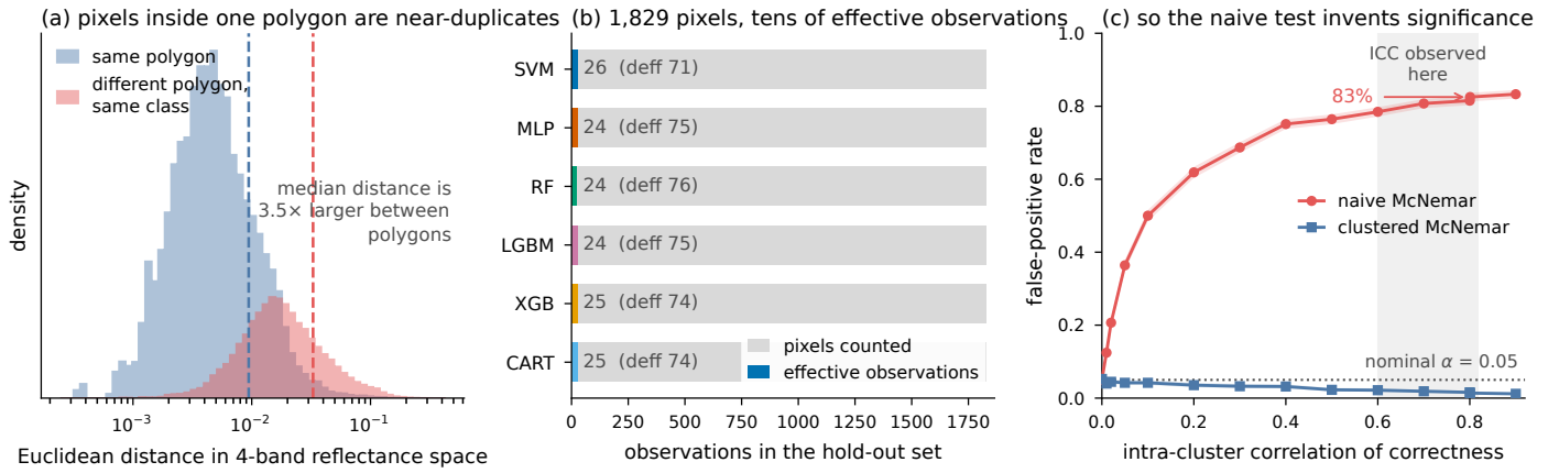
Figure 4. Why the model comparison has to be cluster-aware, in three measured steps. (a) Pixels inside one digitised polygon are near-duplicates of one another: for pairs of pixels of the same class, the median distance in the four-band reflectance space is 3.5 times larger between polygons than within one. (b) The 1,829 validation pixels are therefore worth only 24 to 26 effective observations, a design effect of 71 to 76. (c) A test that assumes independence over-rejects accordingly. Under a null in which two classifiers have identical expected accuracy, the false-positive rate of the naive McNemar test climbs with the intra-cluster correlation of correctness and reaches 82.5% at the value observed here, while the cluster-corrected test of Durkalski et al. [21] stays at or below the nominal 5%. Both tests are calibrated at zero correlation, which is what validates the two implementations. Four thousand null replicates per point; bands are 95% binomial intervals.
