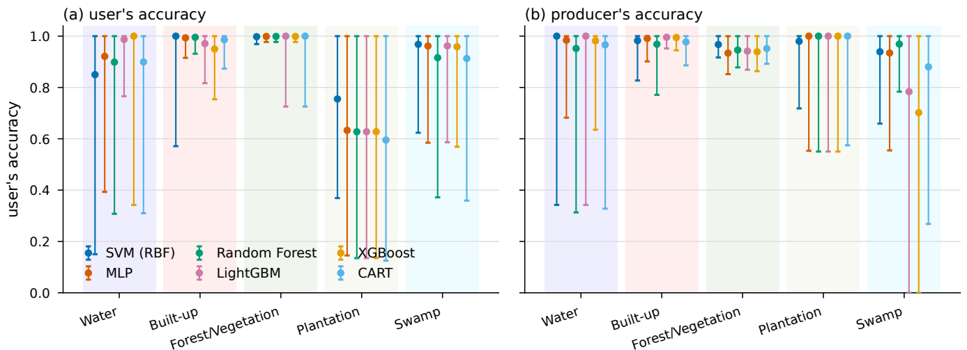
Figure 9. Per-class user's (a) and producer's (b) accuracy for each model, with 95% confidence intervals from the area-weighted estimator.
