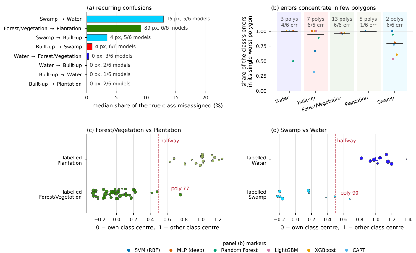
Figure 12. Where the misclassification is. (a) Recurring confusions: for each ordered class pair, the median across models of the share of the true class assigned to the other. (b) For each class and model, the share of that class's validation errors falling inside its single worst polygon. (c, d) Position of each validation polygon on the axis joining the two class centroids in the z-scored four-band feature space, where 0 is the centre of the labelled class and 1 the centre of the class it is confused with.
