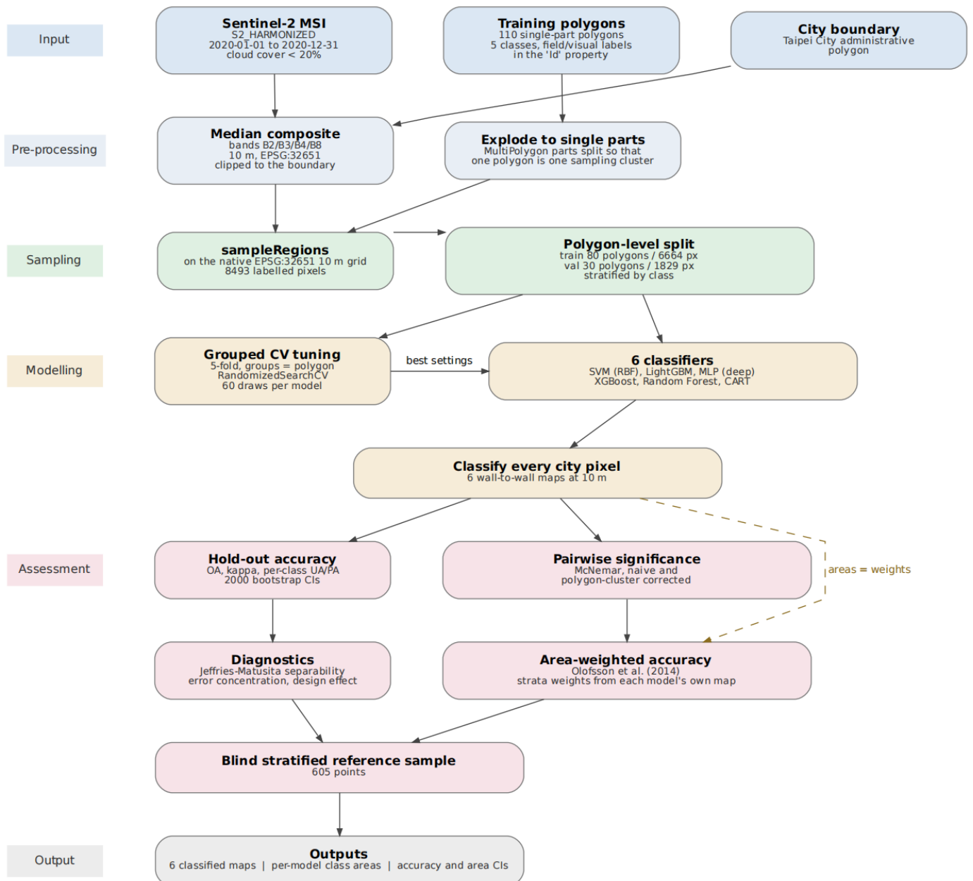
Figure 2. Methodology. Processing runs top to bottom through six stages. Counts inside the boxes are read from the analysis outputs. The dashed feedback path marks the one circularity in the design: the stratum weights W_i of the area-weighted estimator are the mapped class areas, so each model must be assessed against a sample stratified by its own map.
