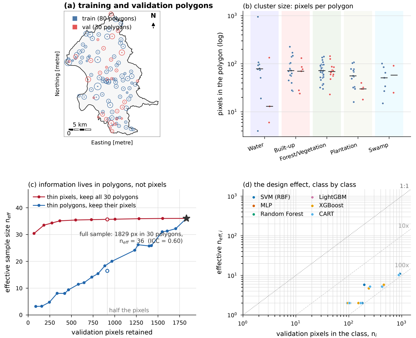
Figure 3. Sampling design and effective sample size. (a) The 110 training polygons, 80 training and 30 validation; ring size is proportional to pixel count. (b) Pixels per polygon by class and split, log scale. (c) The cost of clustering: thinning pixels within polygons (red) against removing whole polygons (blue). (d) The design effect class by class and model by model.
