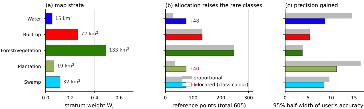
Figure A1. Design of the independent reference sample. (a) Stratum weights W_i . (b) Proportional allocation against the allocation used, which raises each rare class to a floor of 75 points. (c) The resulting 95% half-width of the user's accuracy estimate at the prior accuracy assumed for each class.
