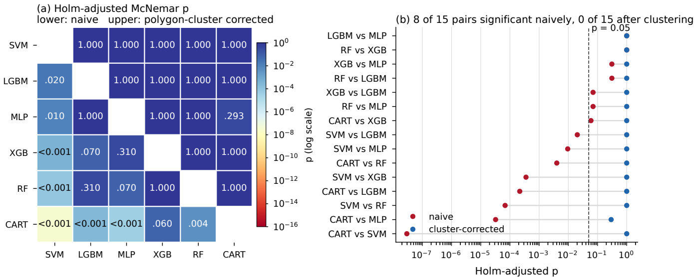
Figure 10. Pairwise significance. (a) Holm-adjusted McNemar p -values for all fifteen model pairs; the lower triangle is the standard pixel-level test, the upper triangle the cluster-corrected test of Durkalski et al. [21]. Colour is on a log scale. (b) The same fifteen comparisons as a paired dot plot, naive against cluster-corrected, with the 0.05 threshold marked.
