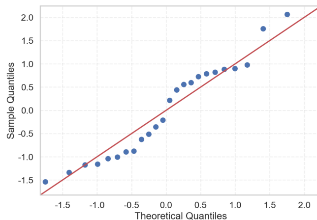
Figure 3. Residual Q–Q plot.
