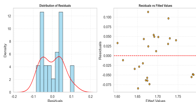
Figure 2. Residual distribution diagnostics.
