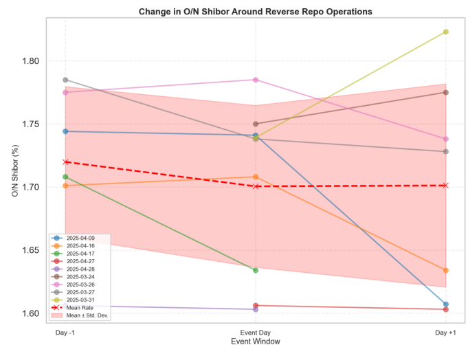
Figure 1. Average change in the overnight rate within the event window.
