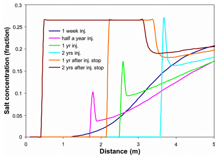
Figure 5. Salt concentration profile versus distance from the borehole after dry CO 2 injection following a freshwater pre-flush (reproduced from [25]).
