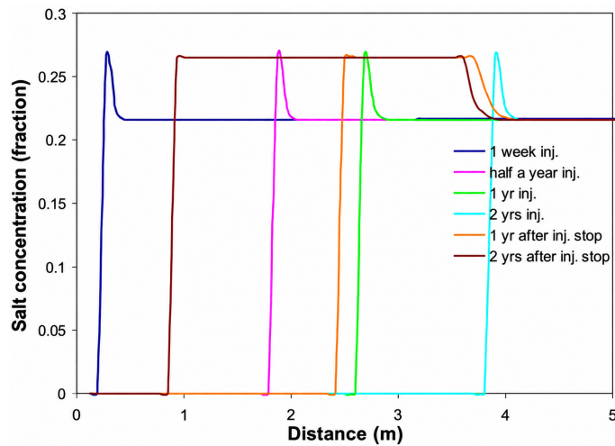
Figure 4. Salt concentration profile versus distance from the borehole after dry CO 2 injection without pre-flush (reproduced from [25]).
