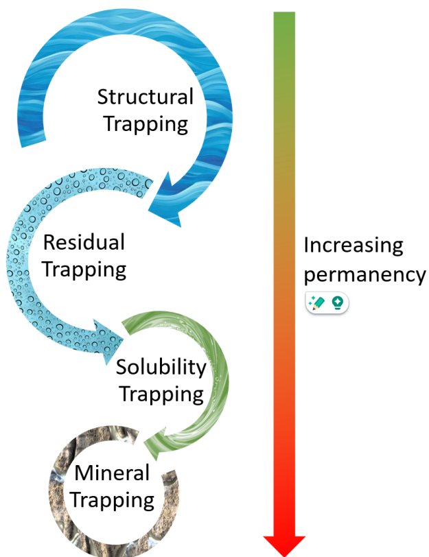
Figure 1. Contribution of different trapping mechanisms and permanency of storage.
