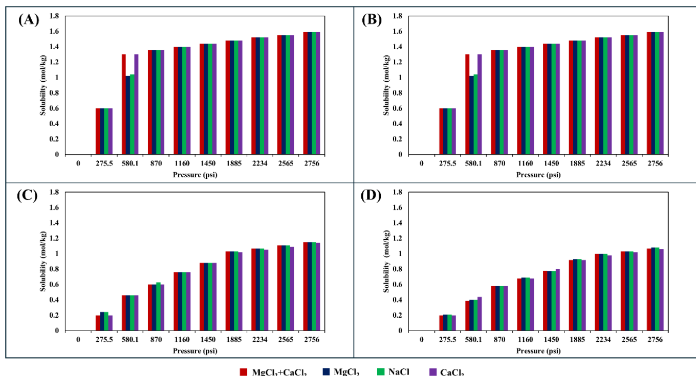
Figure 3. CO 2 solubility in 1000 ppm brines at (A) 25 °C, (B) 60 °C, (C) 80 °C, and (D) 100 °C, plotted from data reported in [76].
