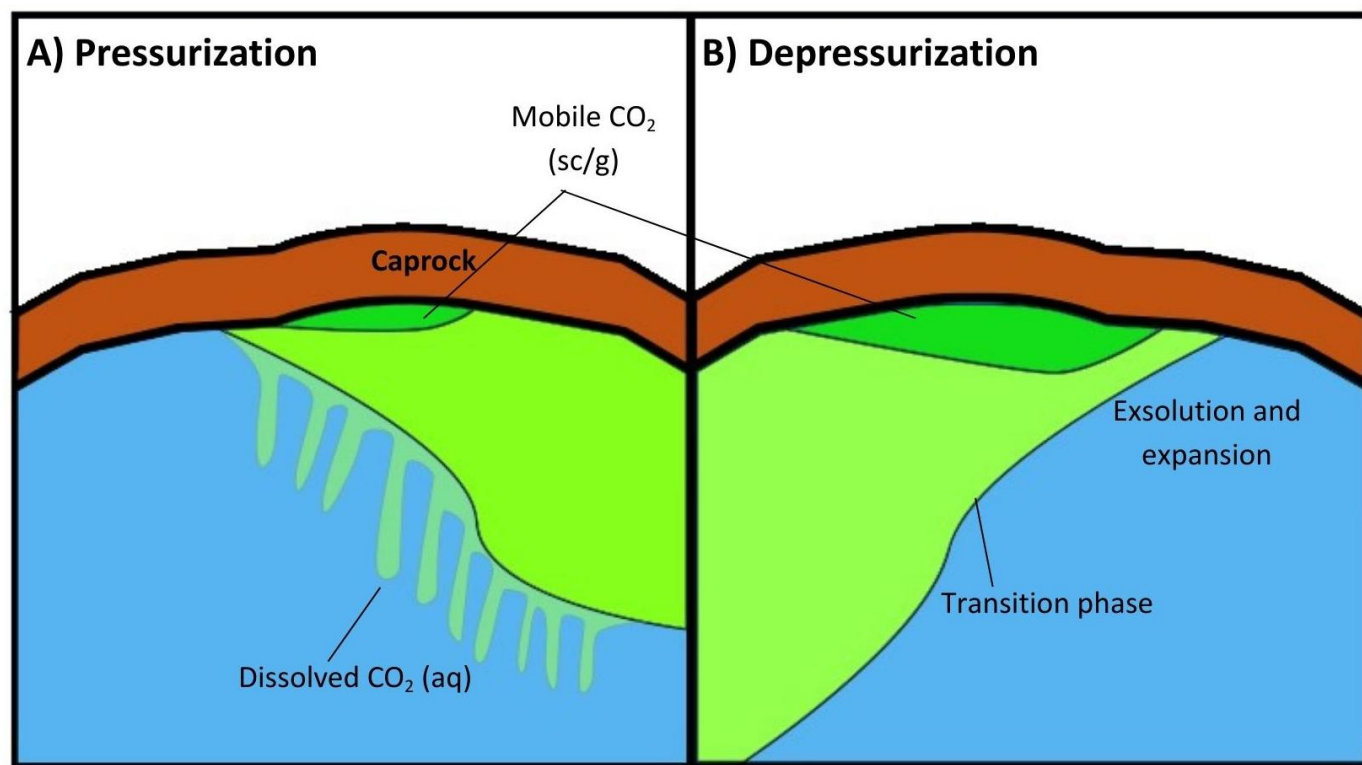
Figure 2. State of CO 2 after injection, undergoing geochemical activity, and the impact of pressure on trapping: (A) CO 2 without depressurization and (B) evolution with depressurization (modified from [28]).
