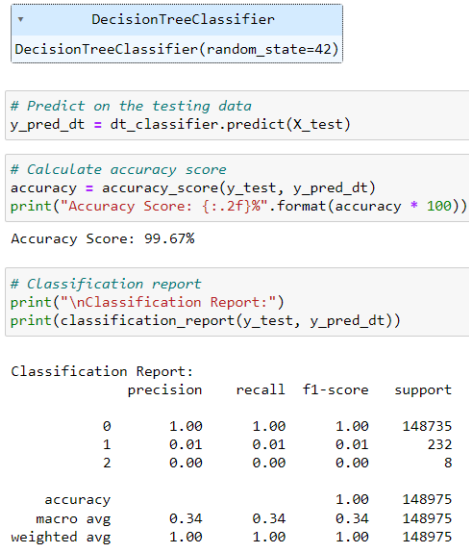
Figure 12. Evaluation Performance of Decision Tree Classifier.
