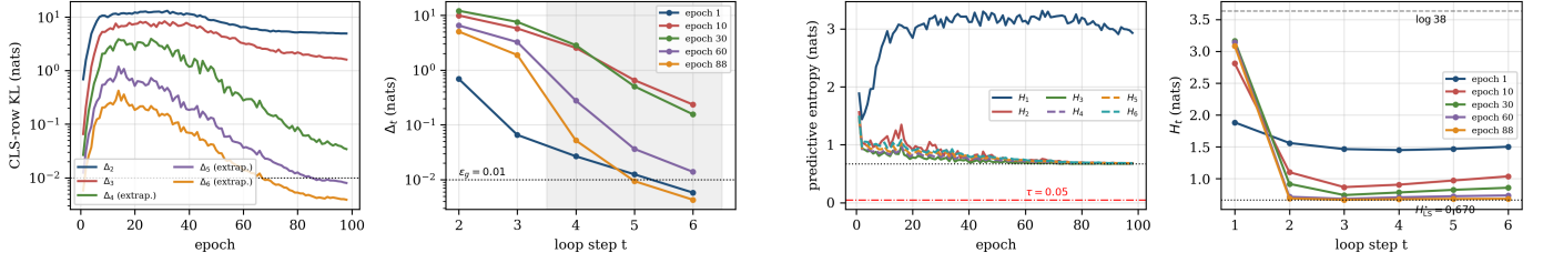
Figure 6. Graph and output dynamics of LoGA-logprob on PlantVillage. Left pair: CLS-row graph change \Delta_t (log scale) (a) across epochs and (b) across loop steps at the selected checkpoint; dotted line \epsilon_g = 0.01 . Right pair: predictive entropy H_t (a) across epochs and (b) at the selected checkpoint; the dotted line is the label-smoothing level H_{LS}^* = 0.671 (Eq. 14) and the red dash-dot line the default entropy threshold \tau = 0.05 , which lies below it and is not reached.
