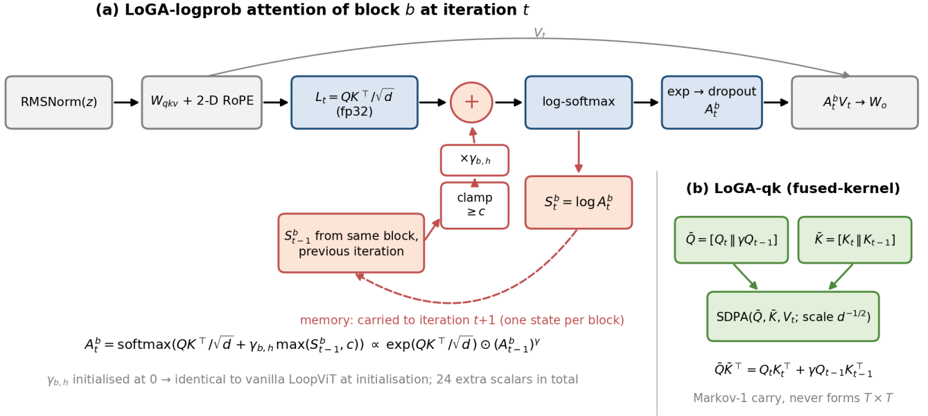
Figure 3. The LoGA attention module. (a) Log-prob carry (primary): the query-key logits L_t of block b are computed in fp32, and the block’s own log-attention graph from the previous iteration, S_{t-1}^b , is floored at c , scaled by the learnable per-head gate \gamma_{b,h} and added before the log-softmax (Eq. 6). The new graph S_t^b = \log A_t^b is stored and carried to the next iteration (dashed). (b) QK carry: the previous queries and keys are concatenated along the head dimension so a fused scaled dot-product attention (SDPA) kernel computes Eq. (11) exactly (Proposition 3).
