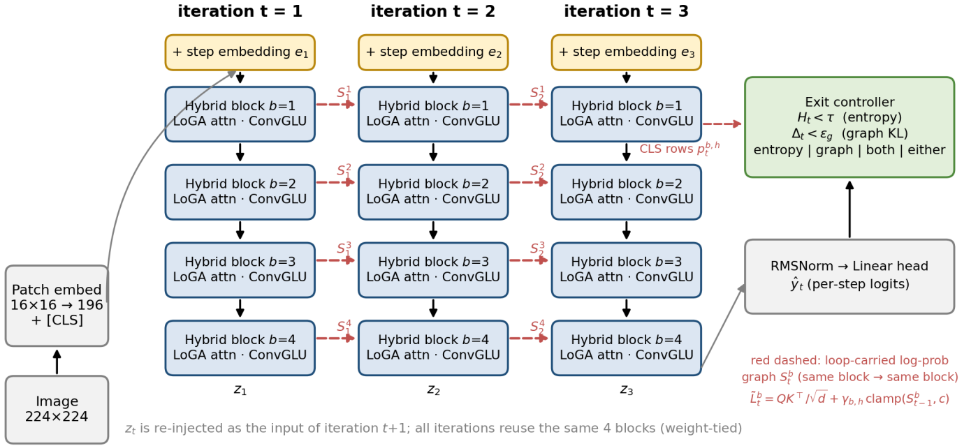
Figure 1. Overview of the LoGA architecture (a looped vision transformer with Loop-Carried Graph Attention). The same four hybrid blocks are applied at every iteration (weight-tied). Each block carries its own attention graph S_t^b to itself at the next iteration (red dashed), where it acts as a tempered prior on the query-key logits. CLS-attention rows feed a graph-stability signal \Delta_t which, together with the predictive entropy H_t , can drive per-sample dynamic exit.
