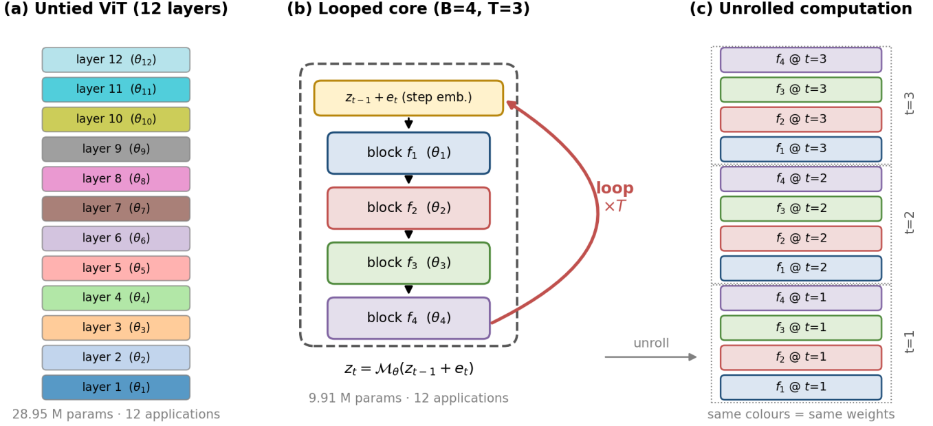
Figure 2. The loop. (a) An untied ViT uses a different set of weights \theta_\ell for each of its 12 layers (28.95 M parameters). (b) The looped core of LoGA holds only B = 4 blocks f_1, \dots, f_4 ; after adding the step embedding e_t , the same four blocks are applied again at every iteration, z_t = \mathcal{M}_\theta(z_{t-1} + e_t) (9.91 M parameters). (c) Unrolled over T = 3 iterations, the looped core also performs 12 block applications, but block f_b at iteration t and at iteration t + 1 is the same function. This is what makes it meaningful to carry the attention graph of f_b from one iteration to the next.
