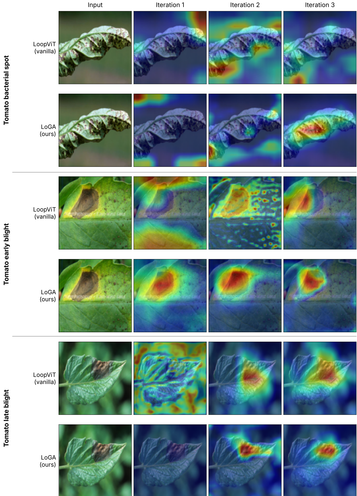
Figure 7. Per-iteration Grad-CAM for three tomato diseases of PlantDoc. For each class, the top row is vanilla LoopViT and the bottom row is LoGA-logprob, on the same test image; columns are the input and the maps of the readouts after iterations 1, 2 and 3 (red = high relevance for the true class).
