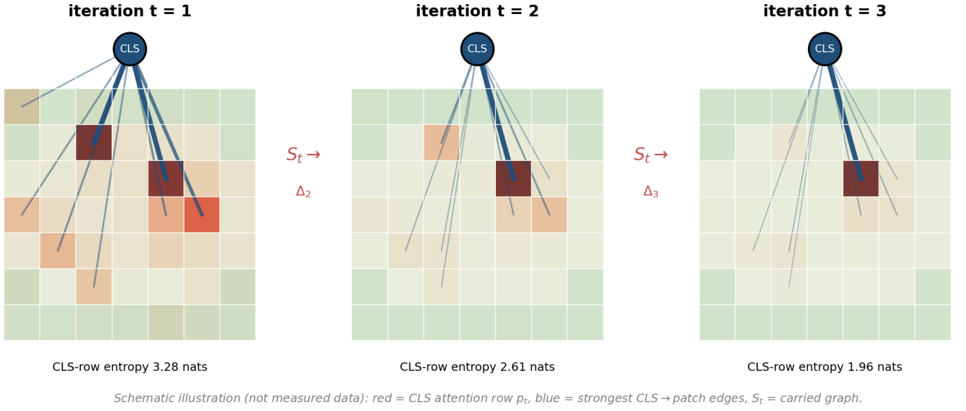
Figure 4. Schematic illustration only (not measured data). Looped graph computation: each panel shows the patch grid of one leaf image with the CLS attention row p_t (red) and the strongest CLS \rightarrow patch edges (blue) of one block at iterations t = 1, 2, 3 . At t = 1 attention is spread over lesion and background patches. The carried graph S_t (red arrows) acts as a prior at the next iteration, so edges can (hypothetically) concentrate on discriminative lesion patches, the CLS-row entropy falls, and the graph change \Delta_t = \text{KL}(p_t || p_{t-1}) shrinks. \Delta_t is the graph-stability signal of Section 3.9; measured values are reported in Section 5.4, and measured per-iteration saliency maps in Section 5.5.
