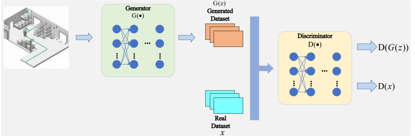
Figure 4. GANs Network Architecture Diagram.
