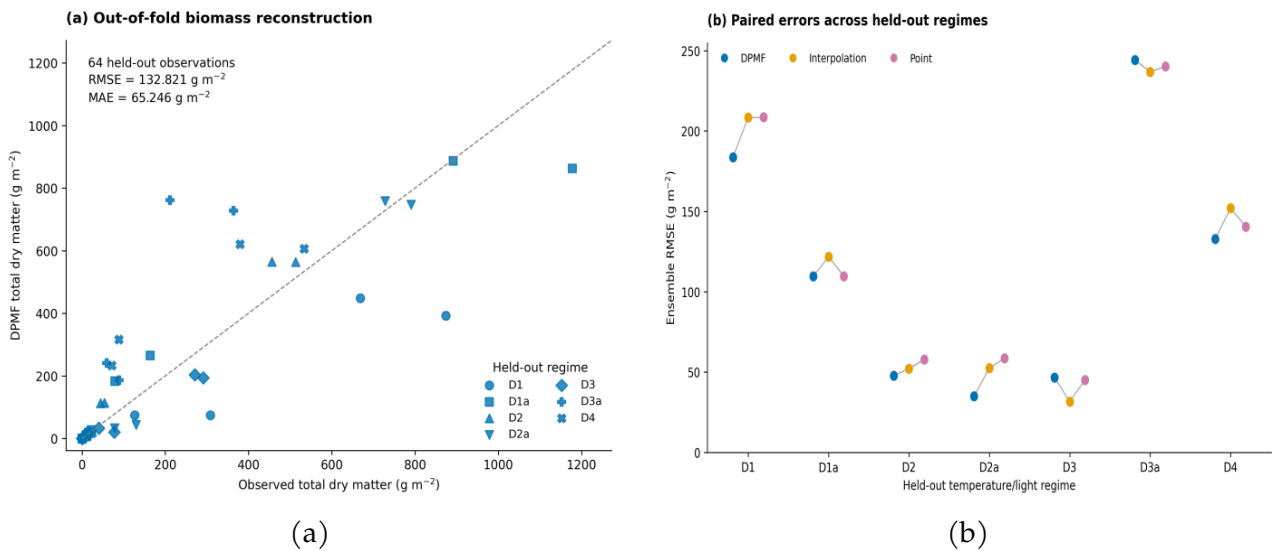
Figure 3. Leave-one-treatment-out evaluation of total-dry-matter reconstruction. (a) Agreement between DPMF predictions and observations for 64 held-out destructive samples; the dashed line is the 1:1 line, and marker shapes distinguish the seven held-out light-temperature treatments. (b) Paired ensemble RMSE of DPMF, Interpolation and Point for each of the seven held-out treatments; lower values indicate better reconstruction.
