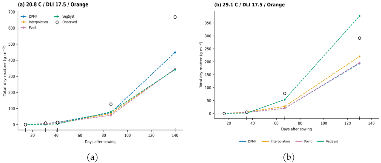
Figure 2. Representative sampling-date total-dry-matter reconstruction under two contrasting temperatures. (a) Orange cultivar at 20.8 °C and DLI 17.5 mol m -2 d -1 . (b) Orange cultivar at 29.1 °C and DLI 17.5 mol m -2 d -1 . Open circles denote observed total dry matter at destructive sampling dates; coloured markers denote predictions from DPMF, Interpolation, Point and VegSyst.
