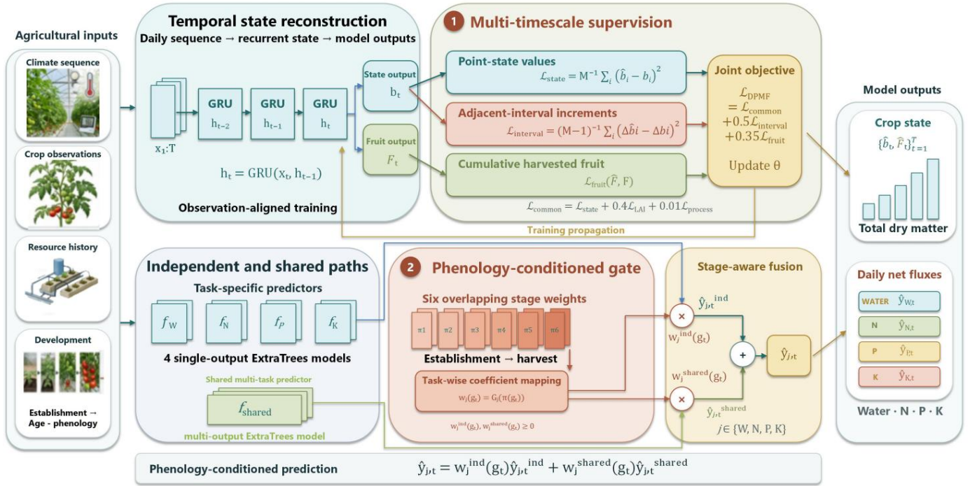
Figure 1. DPMF architecture. The upper path reconstructs total dry matter with a GRU trained on point, interval, cumulative-fruit, leaf area index (LAI) and process-residual terms. The lower path combines independent and shared ExtraTrees predictions through a smooth six-stage phenology gate to estimate daily net water and elemental N, P and K fluxes.
