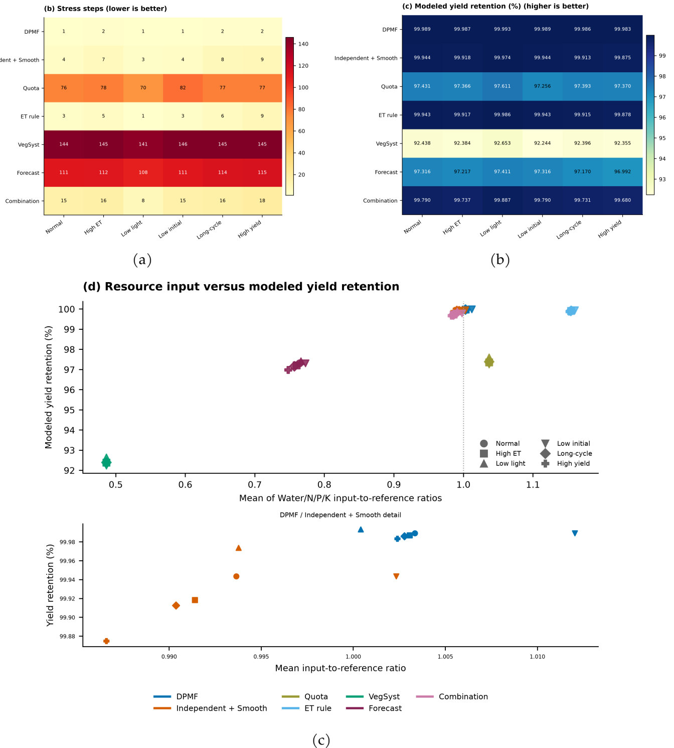
Figure C1. Exploratory scenario-based evaluation of resource-management strategies. (a) Number of stress steps for each strategy-scenario combination; a stress step is a simulation step in which the unmet-demand fraction exceeded 10% for at least one resource (lower is better). (b) Modelled yield retention derived from simulated unmet-demand exposure (higher means lower modelled yield loss); this is a simulation indicator, not measured yield. (c) Mean water/N/P/K input-to-reference ratio versus modelled yield retention for the 42 strategy-scenario combinations; the lower panel enlarges DPMF and Independent + Smooth. The vertical line at a ratio of 1 marks equality between mean normalised input and reference demand. Colours identify strategies and marker shapes identify scenarios.
