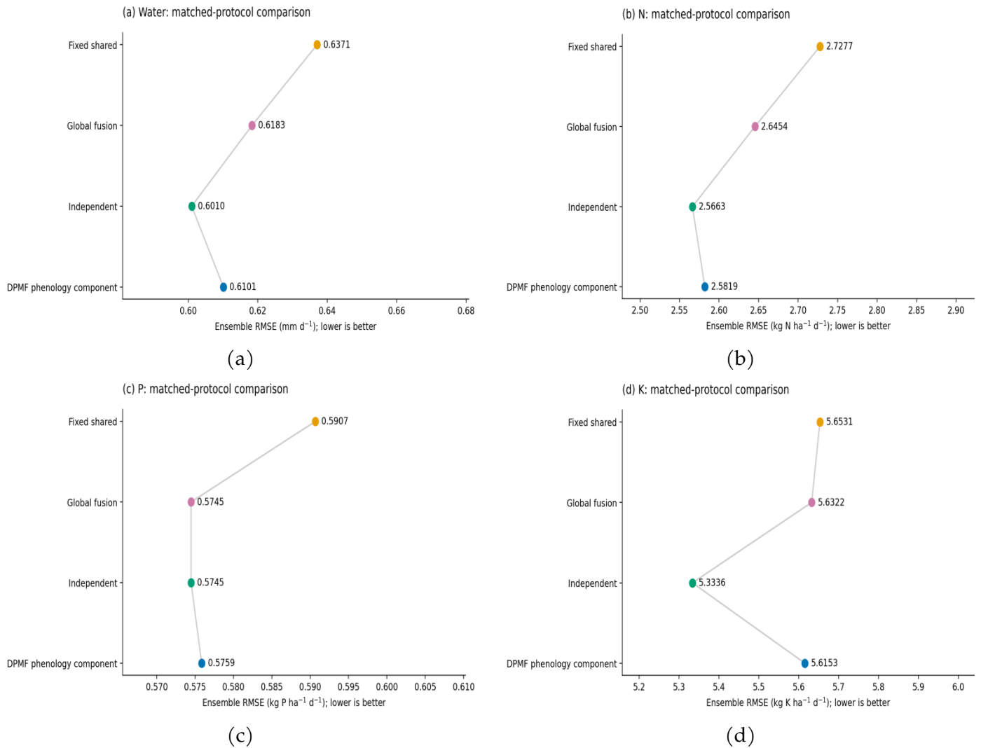
Figure 4. Ensemble RMSE of the four modelling strategies for daily net (a) water, (b) N, (c) P and (d) K fluxes on the 154 Reference test dates. All strategies used the same dates, response definitions, historical inputs and update protocol; lower values are better.
