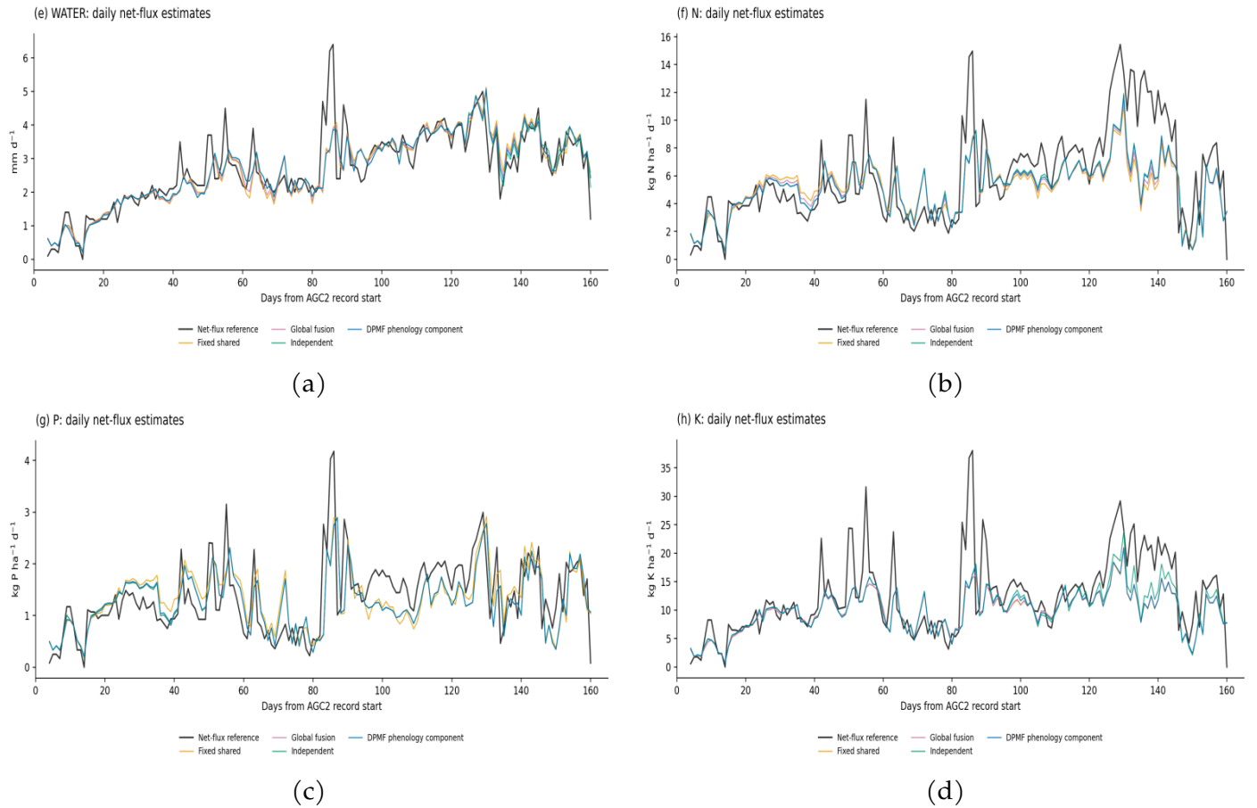
Figure 5. Daily time series of observed and predicted net fluxes over the Reference test period: (a) water, (b) N, (c) P and (d) K. The black line is the reference flux on each of the 154 test dates; coloured lines are five-seed ensemble predictions from Fixed shared, Global fusion, Independent and DPMF. Water is in \text{mm d}^{-1} , and N, P and K are in elemental \text{kg ha}^{-1} \text{d}^{-1} .
