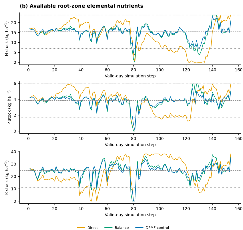
Figure B1. Simulated root-zone water and nutrient dynamics under alternative control rules driven by the same DPMF ensemble predictions. (a) Irrigation actions and simulated available root-zone water storage under Direct, Balance and DPMF control. (b) Simulated available root-zone N, P and K stocks under the same rules. Horizontal dotted, dashed and dash-dotted lines mark 25%, 55% and 85% of the predefined reservoir capacities (low-inventory diagnostic level, initial/feedback target and overflow threshold). Water storage is in mm, and nutrient stocks are in elemental \text{kg ha}^{-1} .
