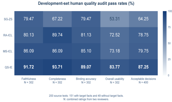
Figure 3. Pooled human audit pass rates (%) on 200 development texts. The first four columns use 302 ratings of 151 target-bearing texts; the last column (acceptable decisions) uses all 400 ratings of the 200 texts and includes correct abstention on 49 non-target texts. The two reviewers rate each output independently, so the number of ratings is not the number of independent texts. The color scale ranges from 0 to 100%.
