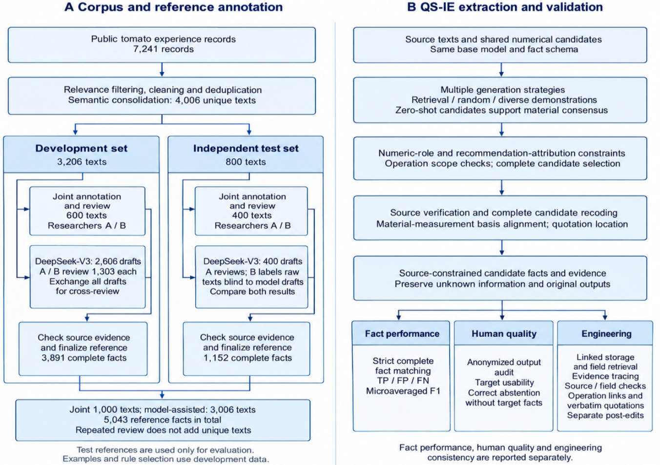
Figure 1. Corpus construction, reference annotation, and QS-IE. (A) The 7241 raw records yield 4006 unique texts, which are split into development and test sets; 1000 texts are jointly annotated and reviewed, and 3006 are annotated with DeepSeek-V3 assistance followed by human review. (B) Complete-candidate selection, source-text verification, and source constraints produce candidate facts with evidence. Test references are used only for evaluation.
