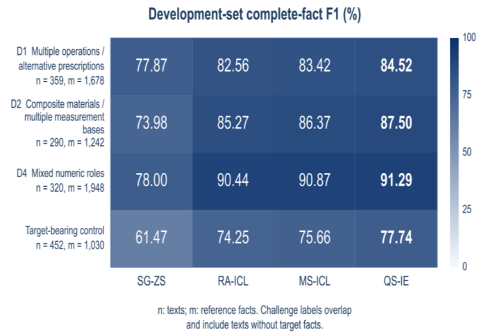
Figure 2. Complete-fact F1 (%) on the development-set challenge scenarios and target-bearing controls. n is the number of texts with each label, and m is the number of reference facts. Challenge labels may overlap and include non-target texts, whereas the controls contain only target-bearing texts. D3 (4 texts, 22 facts) and the 4 target-bearing records with uncertain labels are not plotted. The color scale ranges from 0 to 100%.
