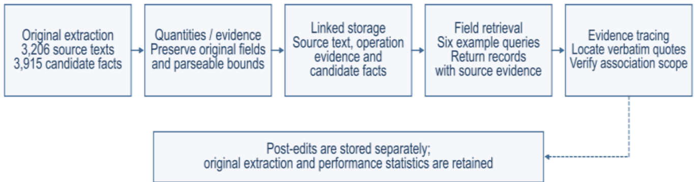
Figure 4. Linked storage, field retrieval, and evidence traceability of development-set candidate facts. The 3915 candidates include both TP and FP. Post-edits are stored separately and do not replace the original extraction outputs or their performance statistics.
