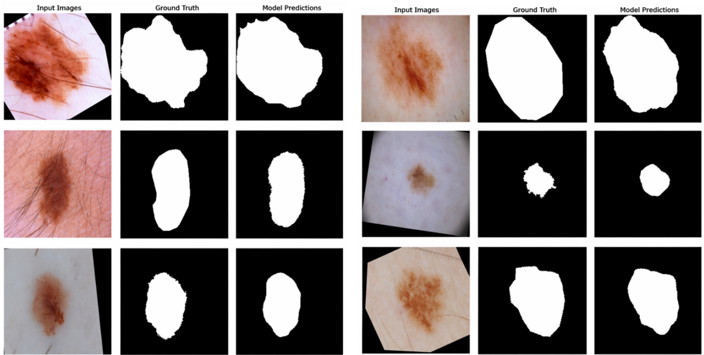
Figure 2. Sample segmentation output from the EfficientNet-UNet model on the ISIC 2018 dataset.
