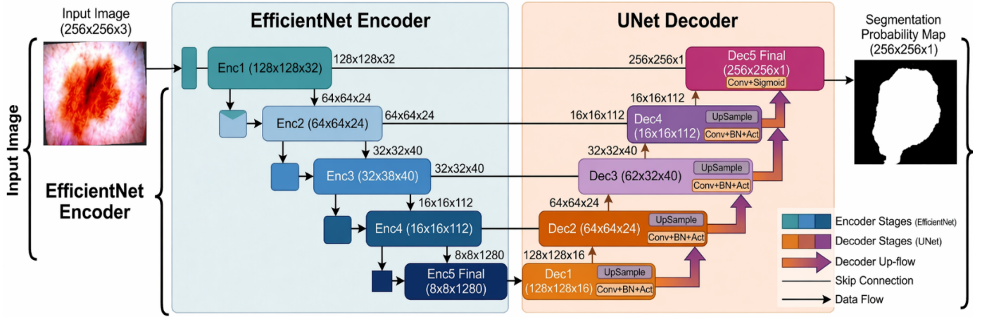
Figure 1. Proposed EfficientNet-UNet architecture, combining an EfficientNet-B0 encoder with a U-Net-style decoder linked by skip connections.
