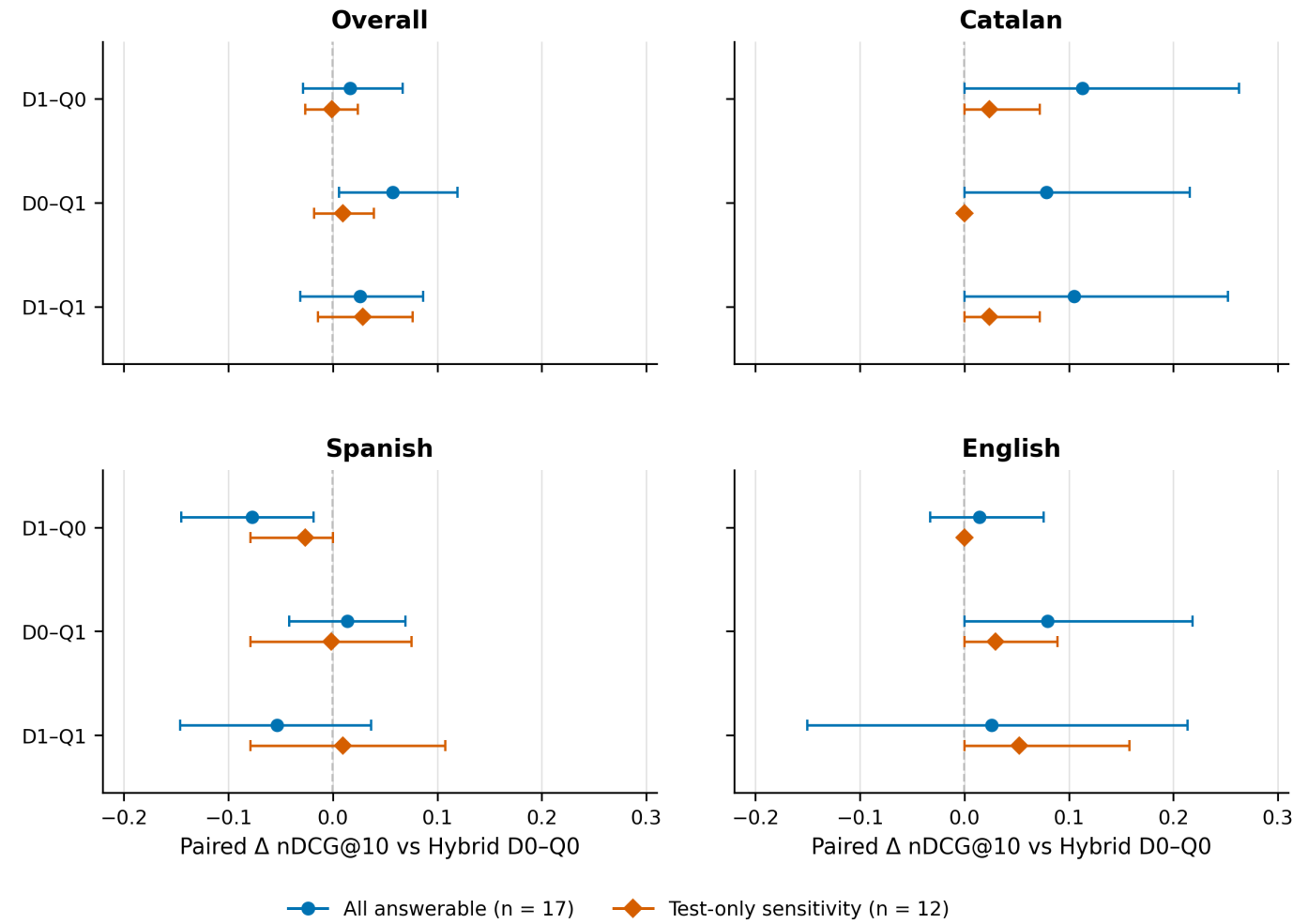
Figure 3. Paired changes in nDCG@10 relative to Hybrid D0-Q0 . Blue circles show the pooled exploratory analysis over 17 answerable intents, and orange diamonds show the held-out test analysis over 12 answerable intents. Error bars represent 95% bootstrap confidence intervals.
