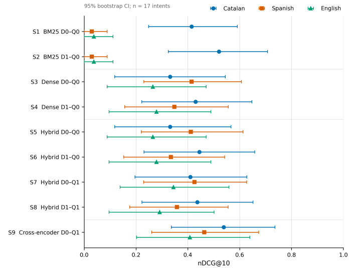
Figure 2. Language-specific nDCG@10 for the nine retrieval configurations in the pooled exploratory analysis. Points show mean effectiveness and horizontal bars show 95% bootstrap confidence intervals over 17 semantic intents. The three language formulations of each intent contain equivalent information needs.
