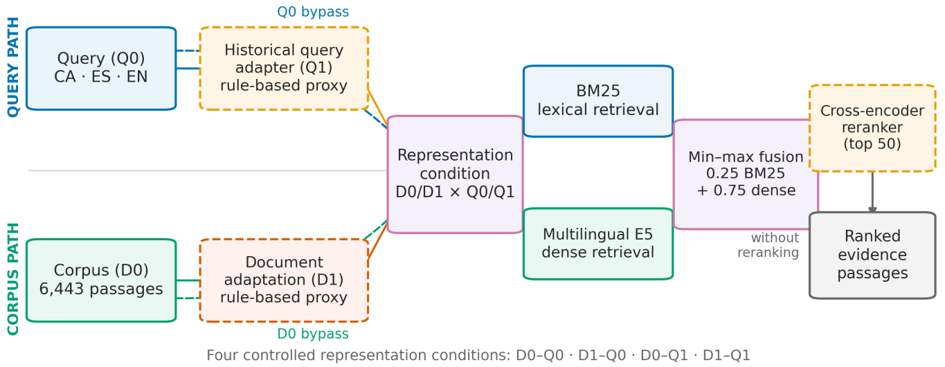
Figure 1. Overview of the HistRAG retrieval pipeline. Contemporary queries in Modern Catalan, Spanish, or English follow either the original Q0 path or the controlled historical-query adaptation Q1 path. Medieval passages are retrieved from either the original corpus D0 or its adapted representation D1 . Each representation condition is evaluated using lexical and multilingual dense retrieval, score-level fusion, and optional cross-encoder reranking.
