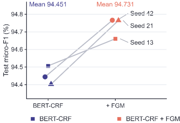
Figure 4. Paired test results. (a) Test micro-F1 for matched BERT-CRF and BERT-CRF+FGM runs for the three fixed seeds; the score axis is truncated to show small differences. (b) Paired changes in precision, recall and F1 for each seed, with the mean \pm sample SD in percentage points. SD bars are not confidence intervals, and no statistical significance is implied.
