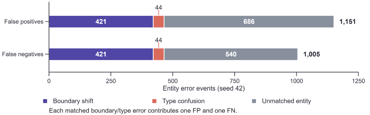
Figure 7. Error composition of the FGM model with seed 42. Absolute FP and FN counts after removing exact matches, then pairing same-boundary type errors and finally overlapping same-type boundary errors. Each paired boundary or type error contributes one FP and one FN, whereas unmatched predictions and missed gold entities contribute only an FP or an FN. Totals are 1,151 FP and 1,005 FN; adding them counts each paired error twice and does not give the number of distinct error events. Error categorization leaves strict entity-level F1 unchanged.
