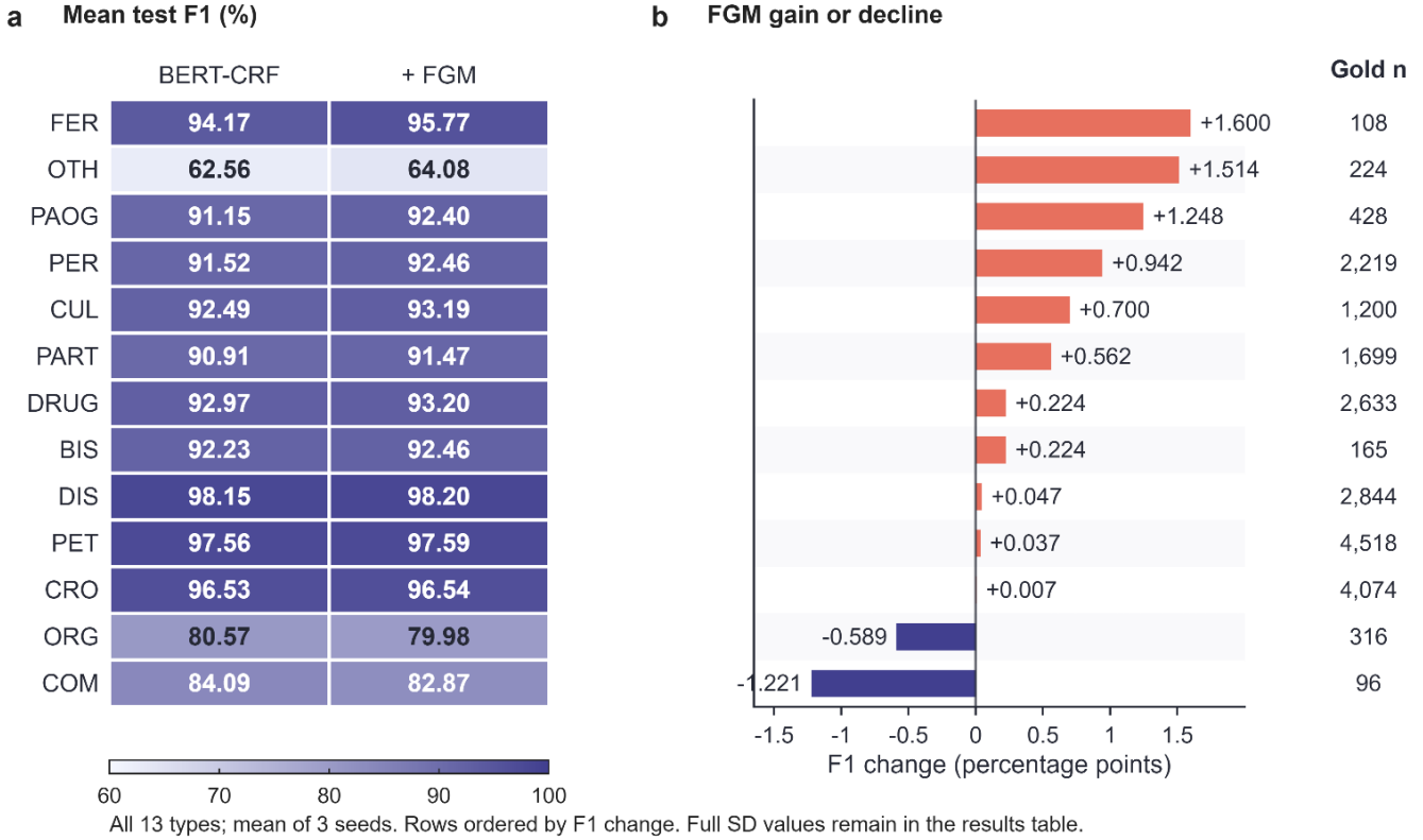
Figure 5. Type-specific test performance and signed FGM gains. (a) Heatmap of mean F1 over three seeds for both models; sample SDs are given in Table 6. (b) Mean F1 of BERT-CRF+FGM minus BERT-CRF in percentage points, with rows ordered by signed change and test gold counts in the right column. No uncertainty interval is derived for the differences, and no multiple-comparison test is reported.
