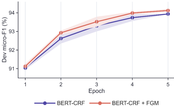
a Development-set learning curves
