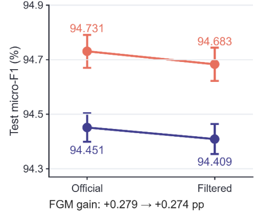
Figure 6. Seen and unseen surface forms and sensitivity to removal of exact duplicate texts. (a) F1 for surface forms seen and unseen among training gold entities, on a percentage axis starting at zero; gains are mean differences in percentage points. (b) Official test micro-F1 and the results after removing test records whose complete text exactly matches a training or development record; the F1 axis is truncated. Bars, points and error bars show means and sample SDs over three seeds. The official and filtered sets contain 5,974 and 5,849 records.
