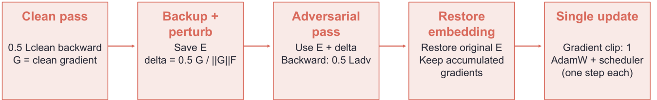
Figure 1. Shared recognition path and FGM training procedure. (a) Subtoken encoding, BERT representation, subtoken-level tag scoring, first-subtoken alignment, CRF decoding and record-level entity indexing. The BIO transition penalty is finite ( -10,000 ) rather than a hard prohibition. (b) A single perturbation of the shared word-embedding matrix during training. Clean and adversarial CRF losses each have a weight of 0.5, and \epsilon = 0.5 . The original embedding is restored before gradient clipping and a single optimizer update. Dropout masks are sampled separately in the two passes. FGM adds no prediction head to the shared inference path.
