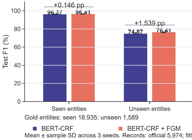
Figure 6. Seen and unseen surface forms and sensitivity to removal of exact duplicate texts. (a) F1 for surface forms seen and unseen among training gold entities, on a percentage axis starting at zero; gains are mean differences in percentage points. (b) Official test micro-F1 and the results after removing test records whose complete text exactly matches a training or development record; the F1 axis is truncated. Bars, points and error bars show means and sample SDs over three seeds. The official and filtered sets contain 5,974 and 5,849 records.
