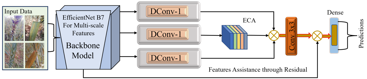
Figure 1. Overview of the proposed network for wheat disease classification.
