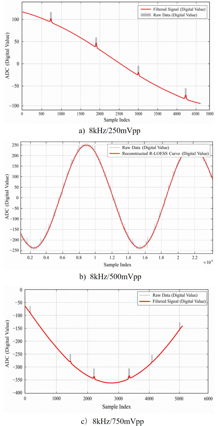
Figure 3. 8 kHz Sinusoidal Excitation: Acquisition, Filtering and Waveform Reconstruction.
