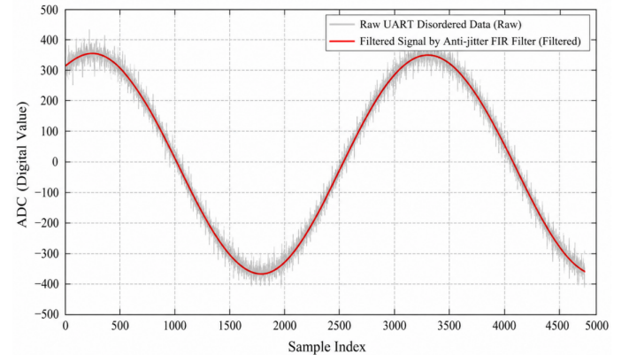
c) 32kHz/750mVpp
