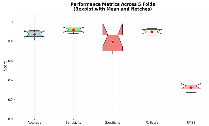
Figure 8. 5-fold cross-validation boxplots with notches and mean markers (red diamonds).
