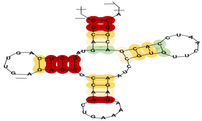
Figure 5. RNA secondary structure (Folding) prediction using RNAfold.
