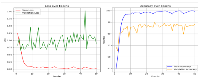
Figure 8. ResNet-50 + ViT.
