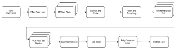
Figure 5. EfficientNet-B0 + ViT Architecture.
