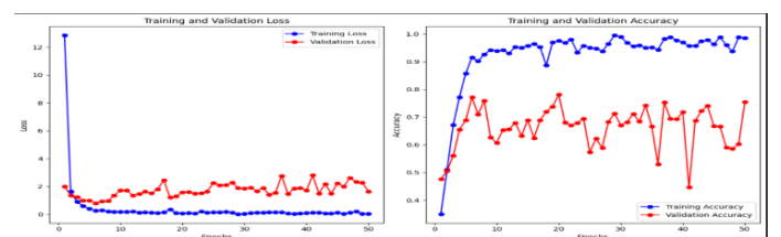
Figure 6. ResNet-50.
