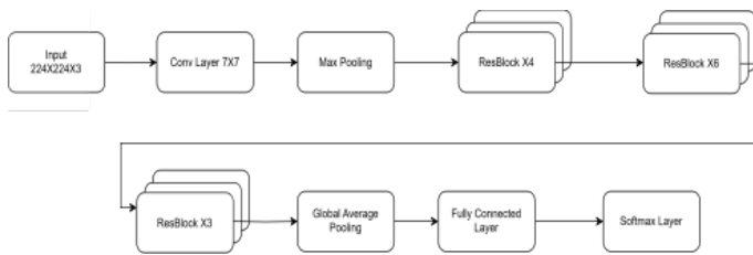
Figure 2. ResNet-50 Architecture.
