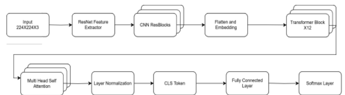
Figure 4. ResNet-50 + ViT Architecture.
