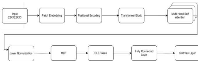
Figure 3. ViT Architecture.
