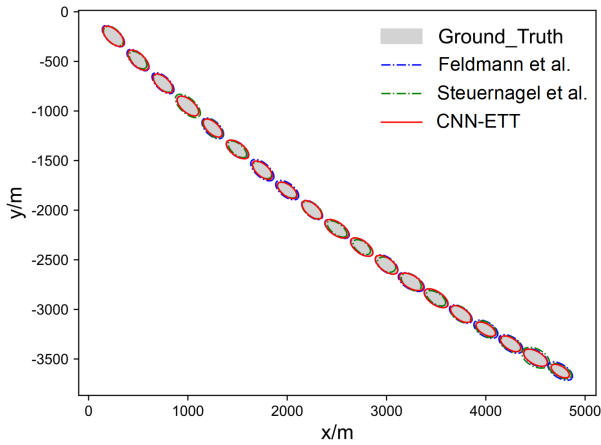
Figure 9. Tracking results under constant acceleration motion.
