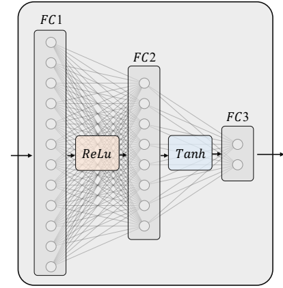
Figure 6. The structure of fully connected layer.
