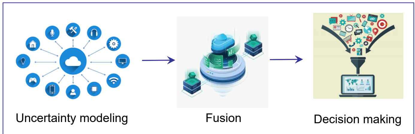
Figure 1. A process of data fusion in the context of evidence theory.
