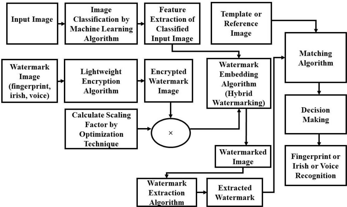
Figure 1. A general framework of biometric authentication using image watermarking.
