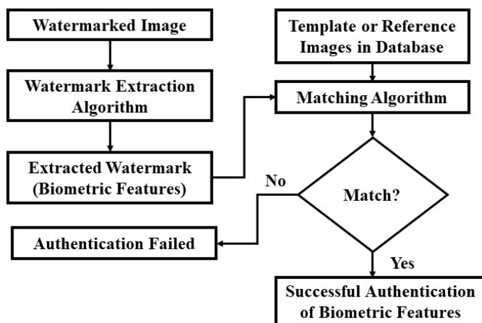
Figure 7. Proposed framework for biometric authentication.
