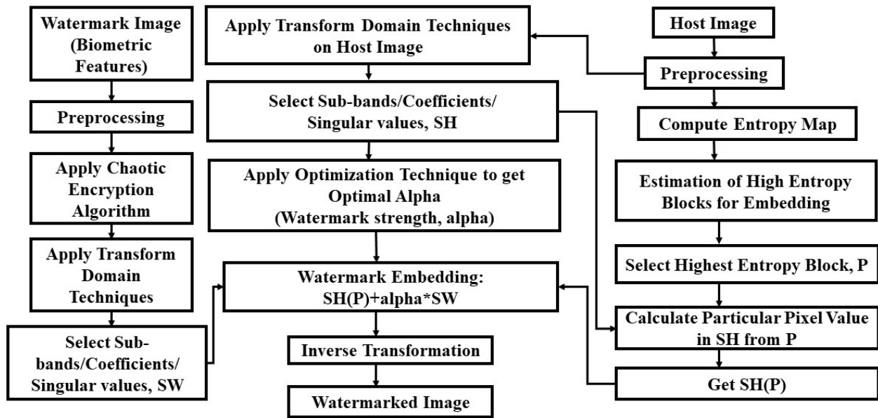
Figure 6. Proposed framework for biometric watermark embedding.
