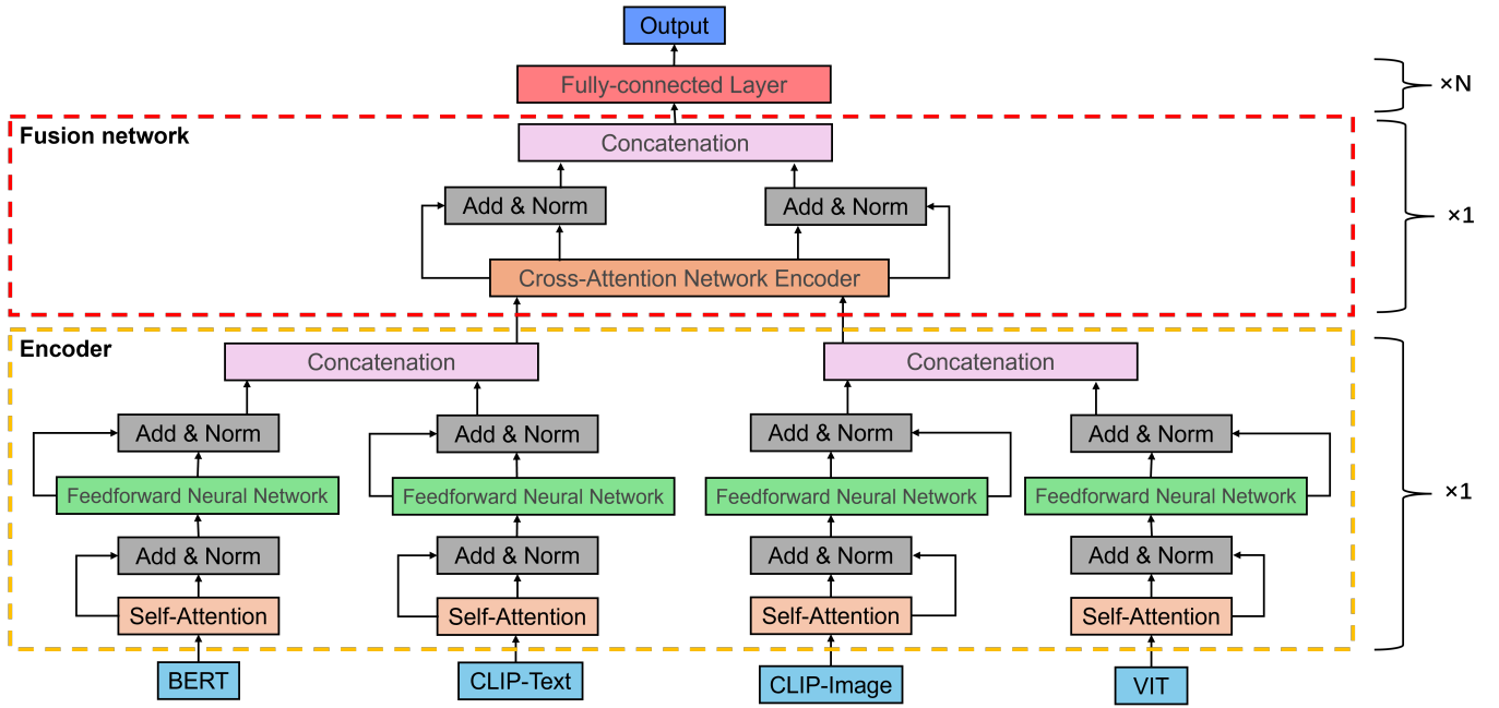
Figure 1. Overview of the proposed multimodal sentiment classification model. It integrates BERT, CLIP (Text/Image), and ViT encoders, and adopt percentage points structured self-attention and cross-attention mechanisms followed by a fully-connected classifier.
