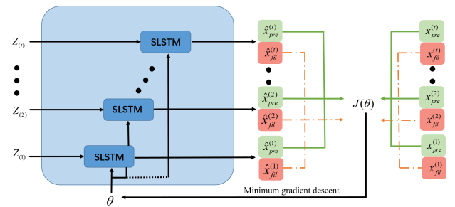
Figure 3. Training architecture of the stacked LSTM fusion network. The input observation sequences Z_{(t)} are processed by the SLSTM blocks to generate predicted ( \hat{x}^{(i)}_{pre} ) and filtered ( \hat{x}^{(i)}_{fil} ) trajectories. These outputs are compared with ground-truth values to compute the cost function J(\theta) , which is minimized using gradient descent to optimize network parameters \theta .
