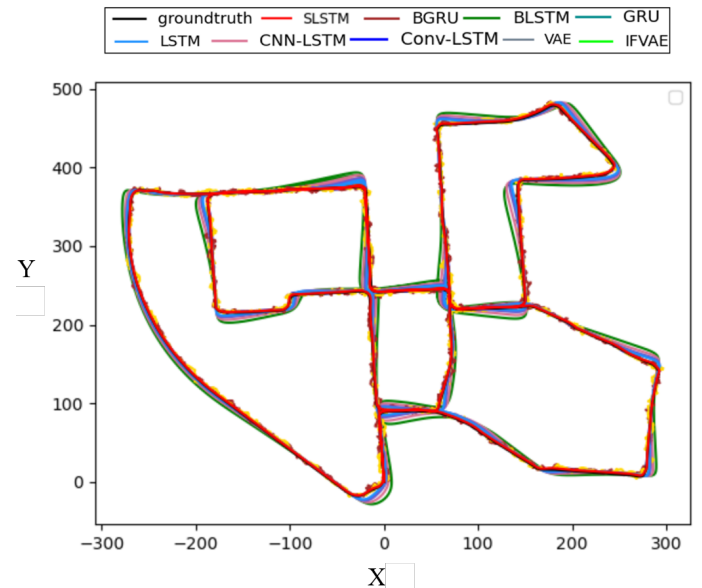
Figure 11. Comparison of different neural network models.
