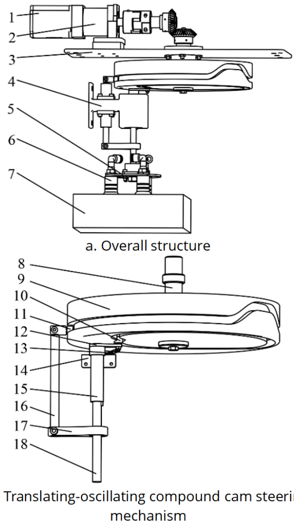
Figure 2. Overall structure of the translating-oscillating compound cam steering mechanism. 1. Stepper motor; 2. Reducer; 3. Fixed upper plate; 4. Fixed frame; 5. End-effector disk; 6. Suction cups; 7. Packaged vegetables; 8. Rotating spindle; 9. Translating-oscillating compound cam; 10. Oscillating roller; 11. Translating roller; 12. Oscillating lever; 13. Spring; 14. Spring fixing frame; 15. Sleeve; 16. Movable shaft; 17. Connecting plate; 18. Shift shaft.
