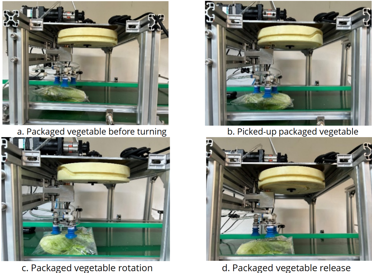
Figure 9. Flipping process of packaged vegetables.
