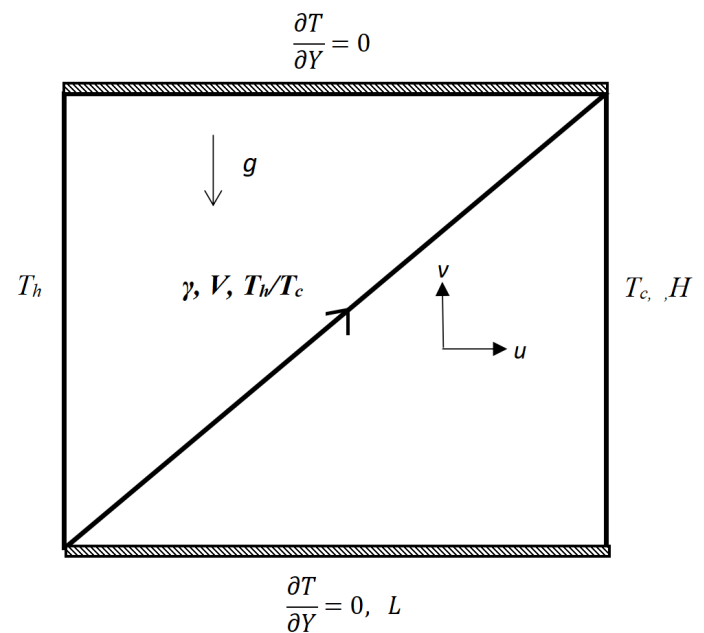
Figure 1. Physical configuration.
