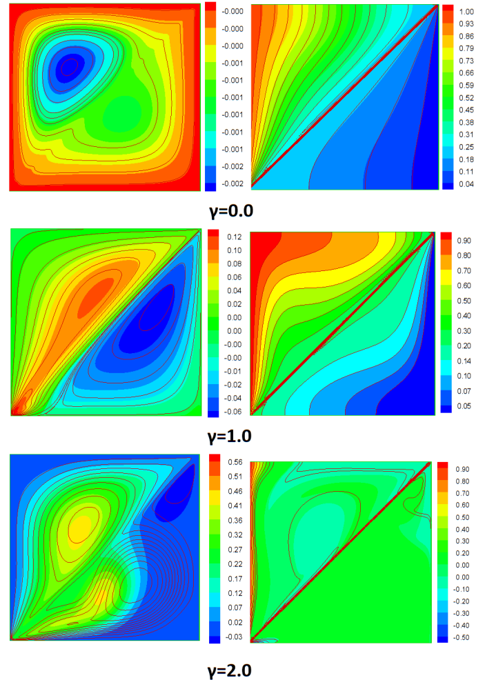
Figure 3. Streamlines and isotherms for different wall speed ratios in the forced convection regime ( Ri=0.1 ) with the heated diagonal moving wall at Ha=10 .
