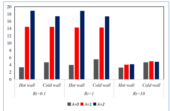
Figure 11. Average Nusselt number profiles for different Richardson number for various wall speed ratios \gamma at Ha=10 .
