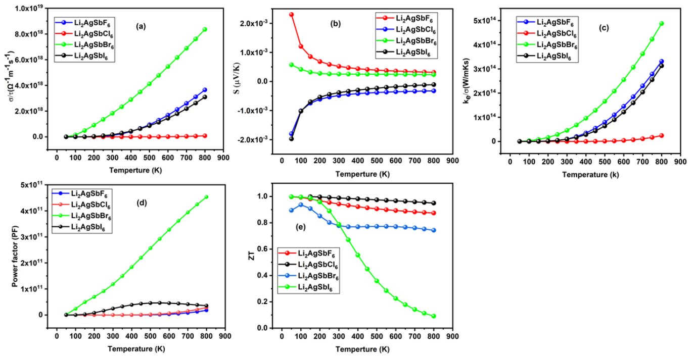
Figure 4. (a) Electrical conductivity, (b) Seebeck coefficient ( S ), (c) thermal conductivity, (d) power factor, and (e) Figure of merit ( ZT ) for \text{Li}_2\text{AgSbX}_6 ( X = \text{F, Cl, Br, I} ).
