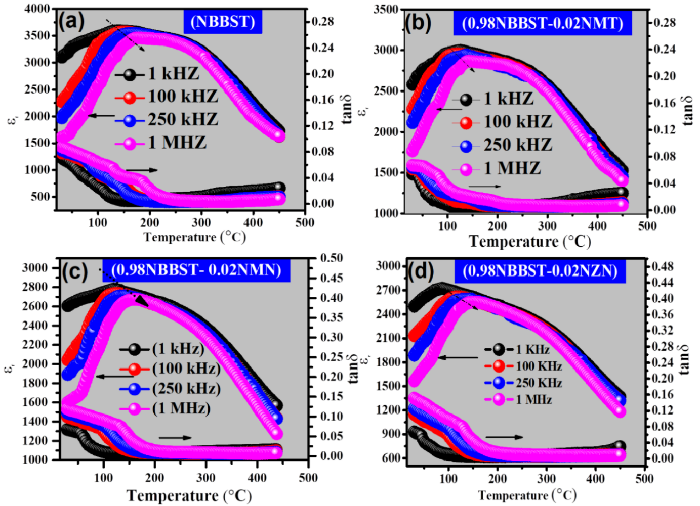
Figure 3. Temperature dependence of dielectric constant ( \epsilon_r ) and dielectric loss ( \tan\delta ) at various frequencies for (a) NBBST, (b) 0.98NBBST-0.02NMT, (c) 0.98NBBST-0.02NMN, and (d) 0.98NBBST-0.02NZN ceramics.
