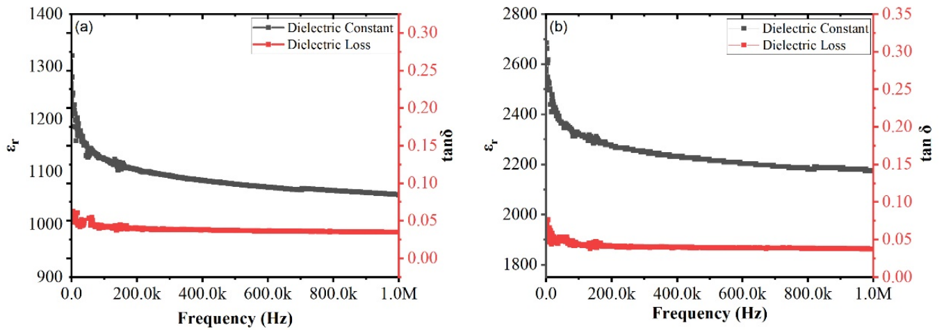
Figure 2. Dielectric permittivity \varepsilon_r and dielectric loss \tan \delta versus frequency (room temperature) for BCZT–SBT ceramics with (a) x = 0 and (b) x = 0.025 .
