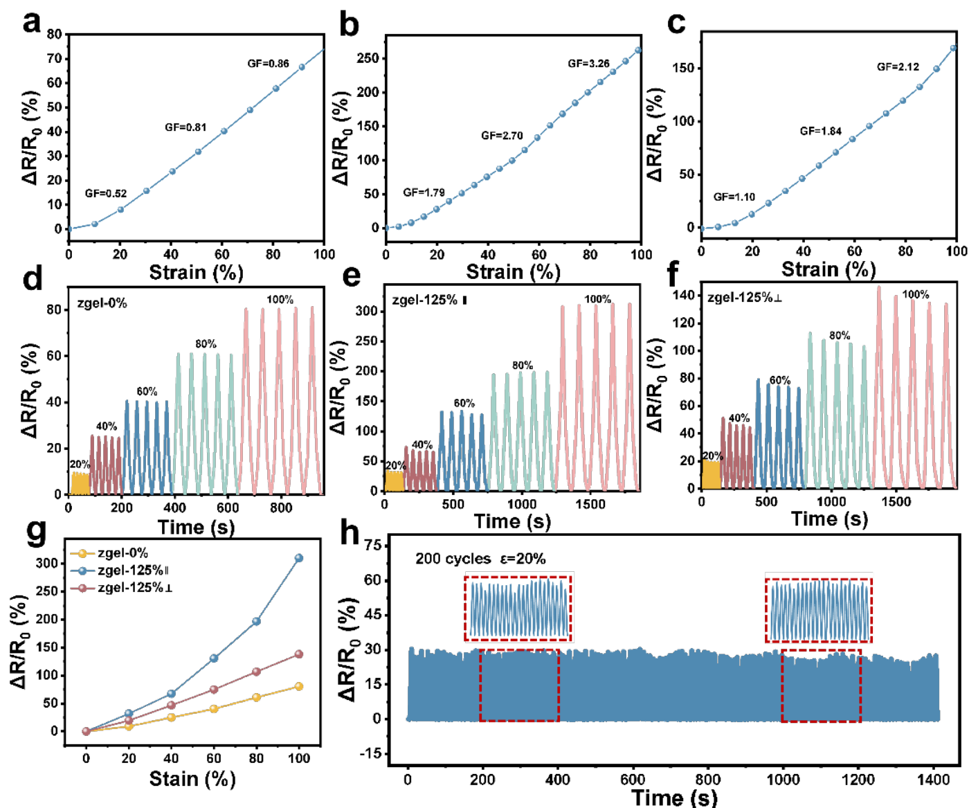
Figure 5. Strain sensors made of zgel-0% hydrogel and zgel-125% (|| and ⊥) hydrogel: (a–c) Variation of relative resistance with strain; (d–f) Relative resistance changes under different strains; (g) Comparison of relative resistance changes; (h) Cyclic stability of zgel-125% ⊥ hydrogel strain sensor after 200 cycles at 20% tensile strain.
