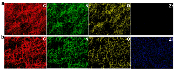
Figure A2. EDS spectra of P(DMAA-AA)-CMC and \text{Zr}^{4+} -P(DMAA-AA)-CMC hydrogels.
