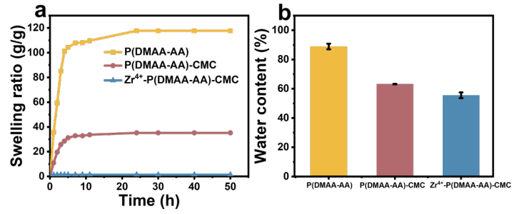
Figure A3. (a) Swelling ratio and (b) water content of P(DMAA-AA), P(DMAA-AA)-CMC, and \text{Zr}^{4+} -P(DMAA-AA)-CMC hydrogels.
