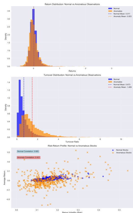
Figure 2. Performance comparison of normal vs anomalous observations.
