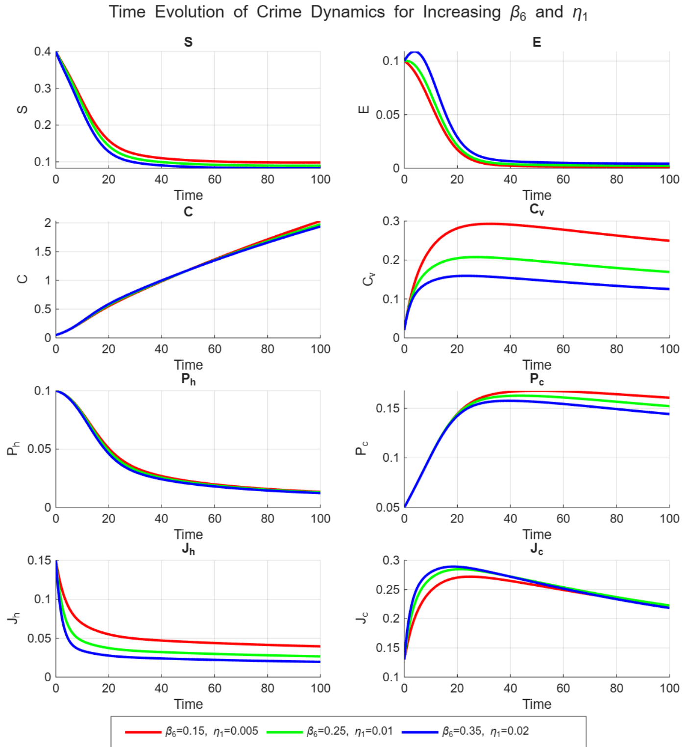
Figure 15. Time evolution of all population compartments for increasing values of the crime–judicial interaction rate \beta_6 and susceptibility parameter \eta_1 . The trajectories correspond to the parameter sets (\beta_6, \eta_1) = (0.15, 0.005) (red), (0.25, 0.01) (green), and (0.35, 0.02) (blue). An increase in \beta_6 and \eta_1 accelerates the depletion of susceptible and honest populations ( S, E, P_h, J_h ), while amplifying criminal and correctional compartments ( C, C_v, P_c, J_c ), indicating enhanced crime propagation under higher exposure and institutional corruption effects.
