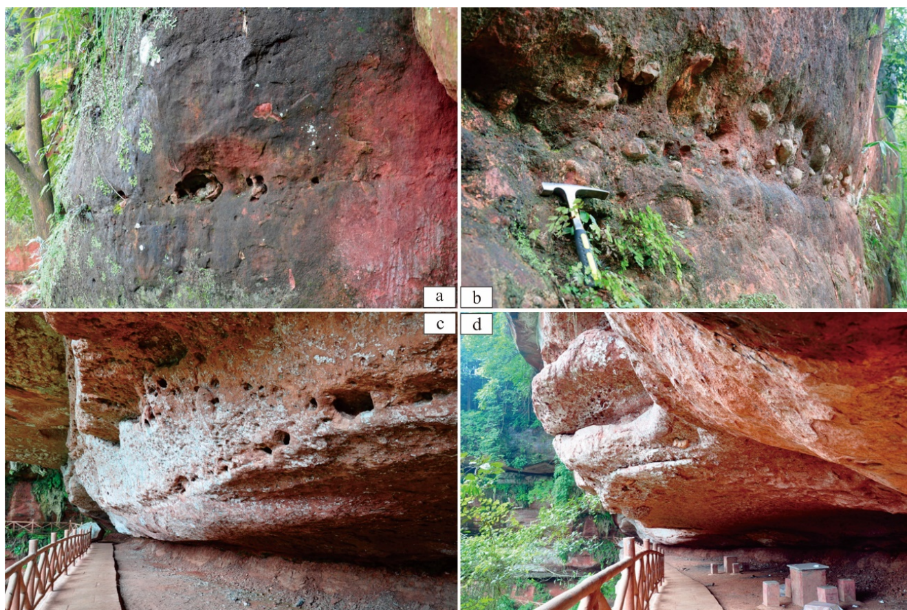
Figure 7. Weathered pebbly sandstone at Guankou scenic area.
