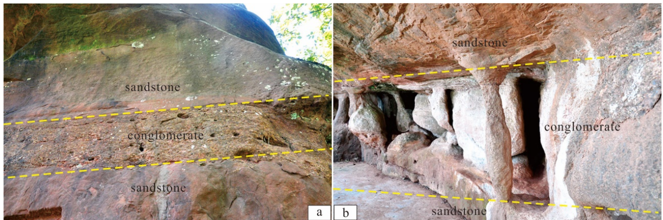
Figure 8. Weathered conglomerate at Bijiaoshan scenic area.
