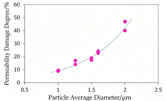
Figure 3. Relationship between particle diameter and permeability damage in injected water.
