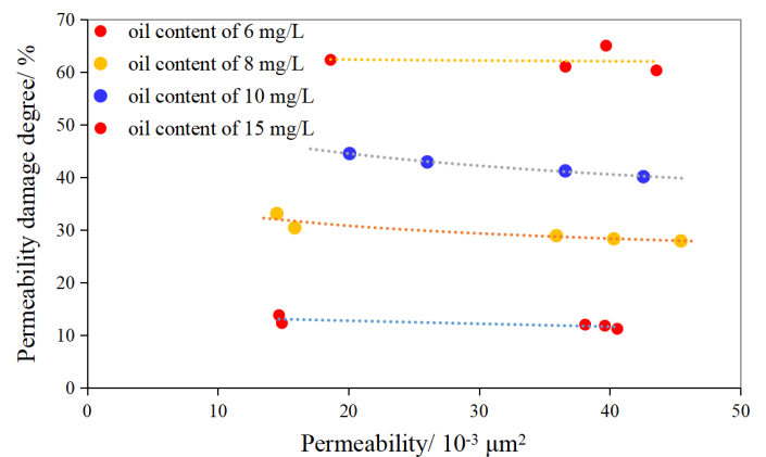
Figure 7. Variation curve of core damage rate with permeability under different oil content.
