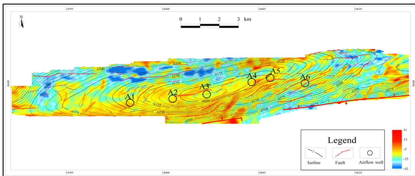
Figure 7. Seismic wave half-broadband attribute plane diagram.
