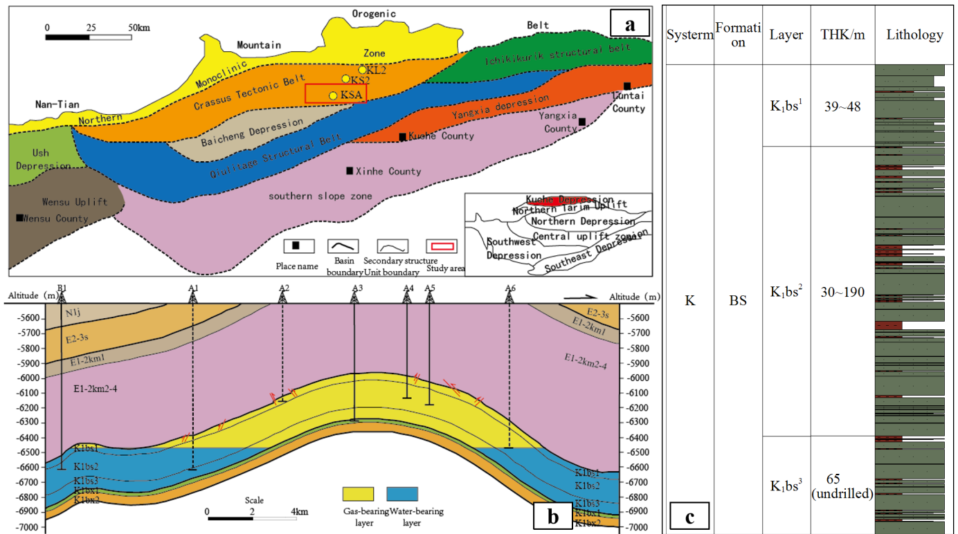
Figure 1. The regional location (a), east-west gas reservoir profile (b) and stratigraphic histogram (c) of Keshen A gas reservoir in Kuqa Depression, Tarim Basin.
