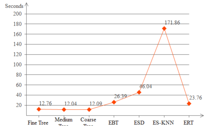
Figure 11. Computational time comparison of classifiers in experiment 3.
