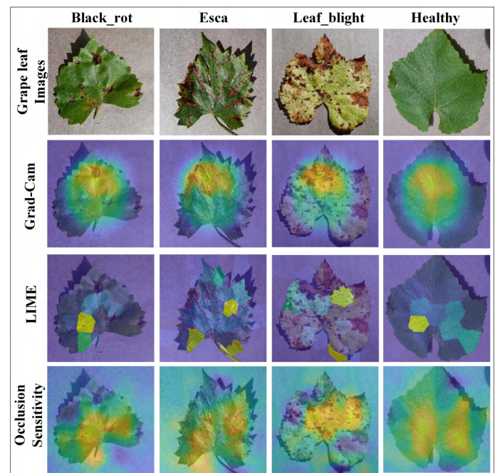
Figure 10. XAI results of the customized CNN network on grape leaf images.
