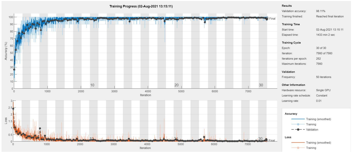
Figure 5. Training performance of the CNN model.
