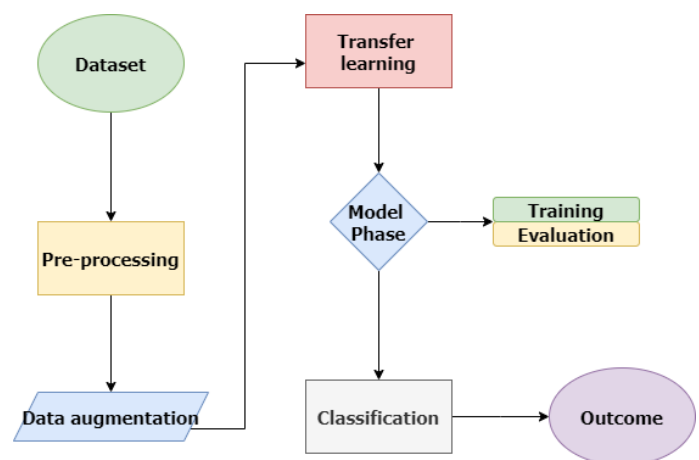
Figure 1. Proposed Model.
