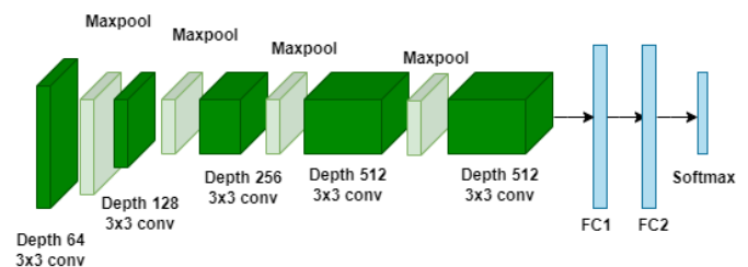
Figure 3. Architecture VGG19.
