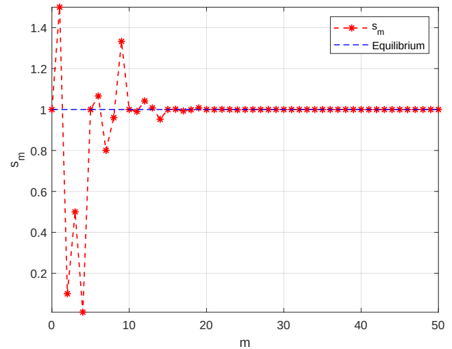
Figure 1. The fixed point \bar{s} = 1 is GAS.
