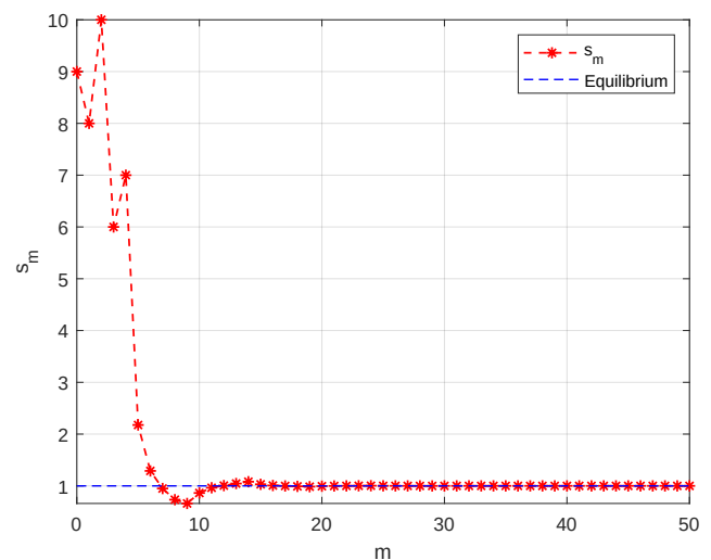
Figure 2. The fixed point \bar{s} = 1 is GAS.
