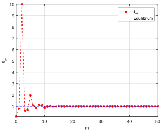
Figure 3. The fixed point \bar{s} = 1 is GAS.
