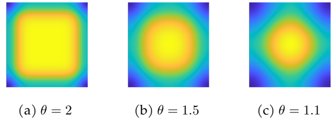
Figure 6. When d_2 = 0.1 < d_2^* and \alpha = 0.05 < \alpha^* , the emergent mussel density patterns ( M ) are presented in panels (a), (b), and (c) for \theta = 2, 1.5 , and 1.1 respectively.
