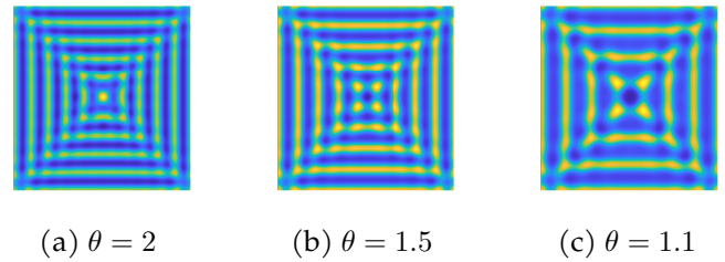
Figure 5. Under critical parameter conditions d_2 = d_2^* and \alpha = \alpha^* , the emergent algae density patterns ( A ) are presented in panels (a), (b), and (c) for \theta = 2, 1.5 , and 1.1 respectively.
