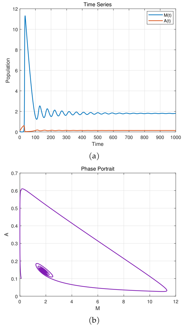
Figure 2. For system (4) with (d_1 = d_2 = 0) , and \alpha > \alpha^* , time series and phase portrait show E^* is asymptotically stable.
