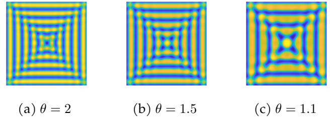
Figure 4. Under critical parameter conditions d_2 = d_2^* and \alpha = \alpha^* , the emergent mussel density patterns ( M ) are presented in panels (a), (b), and (c) for \theta = 2, 1.5 , and 1.1 respectively.
