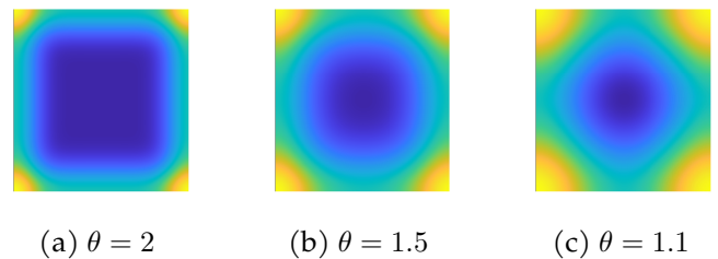
Figure 7. When d_2 = 0.1 < d_2^* and \alpha = 0.05 < \alpha^* , the emergent algae density patterns ( A ) are presented in panels (a), (b), and (c) for \theta = 2, 1.5 , and 1.1 respectively.
