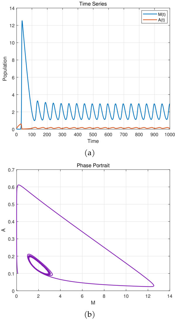
Figure 3. For system (4) with (d_1 = d_2 = 0) , and \alpha < \alpha^* , time series and phase portrait show that a stable limit cycle bifurcates from E^* .
