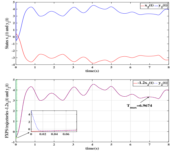
Figure 10. FTPS trajectories of states x_2(t), y_2(t) with \theta = -1.2
