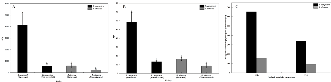
Figure 2. Leaf \Delta G_B (A), MA (B) and change rate of \Delta G_B and MA (C) under saturated and non-saturated water conditions. (Note: Values in the figure are presented as mean ± SE ( n = 3). Based on the results of One-way ANOVA, different lowercase letters are labeled above the error bars for a given parameter when there are significant differences in values of that parameter between different groups at the P ≤ 0.05 level.).
