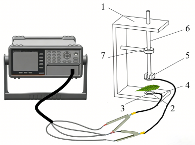
Figure 1. Schematic of the parallel-plate capacitor: 1: bracket, 2: foam board, 3: electrode; 4: wire, 5: iron, 6: plastic bar, 7: fixation clamp.
