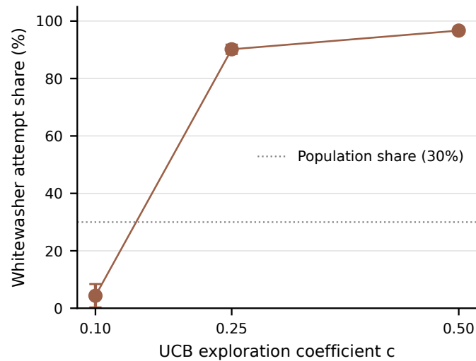
Figure 6. UCB sensitivity with 30% whitewashing workers and no evidence discount. Points are mean attempt shares across ten runs; bars show \pm 1 population standard deviation. The dotted line is population share, not a theoretical decision threshold.
