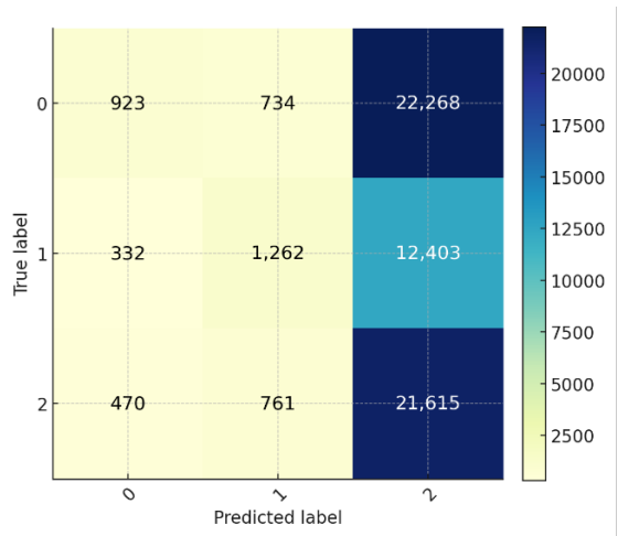
Figure 4. SVM Confusion Matrix (Raw Data).
