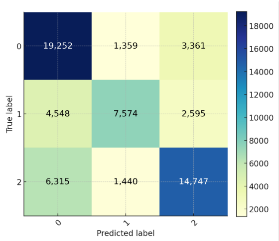
Figure 3. XGBoost Confusion Matrix (Raw Data).
