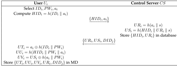
Figure 3. Registration phase for U_i .
