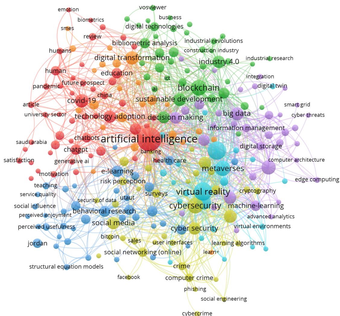
Figure 2. Keyword analysis.
